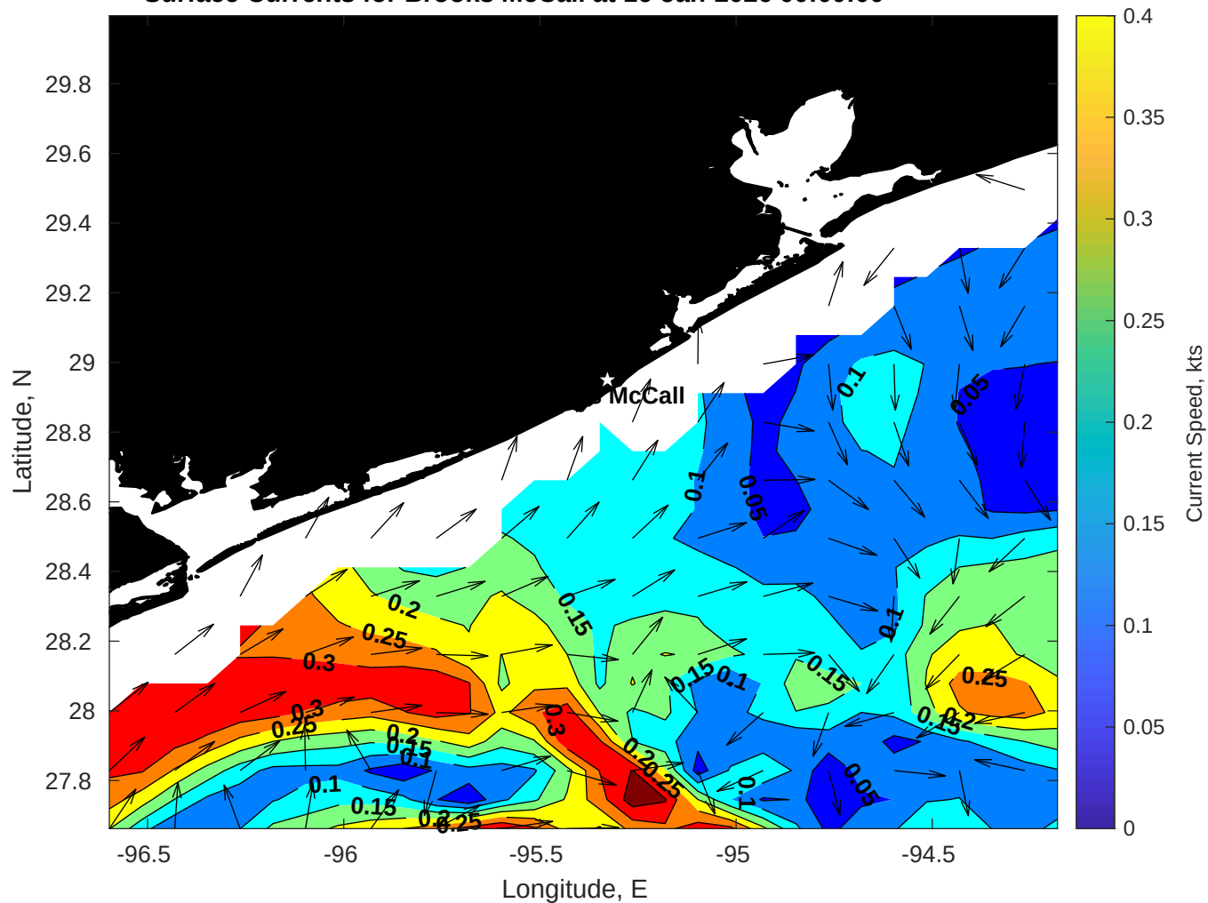
Surface Currents for Brooks McCall at 16-Jan-2026 00:00:00
