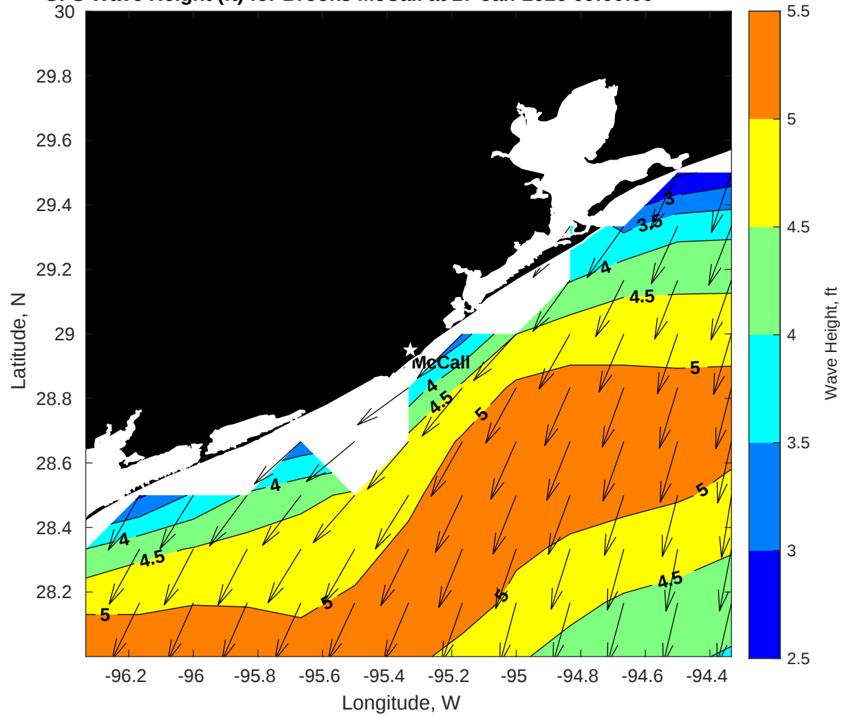
GFS Wave Height (ft) for Brooks McCall at 17-Jan-2026 09:00:00
