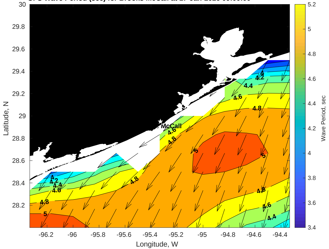
GFS Wave Period (sec) for Brooks McCall at 17-Jan-2026 09:00:00
