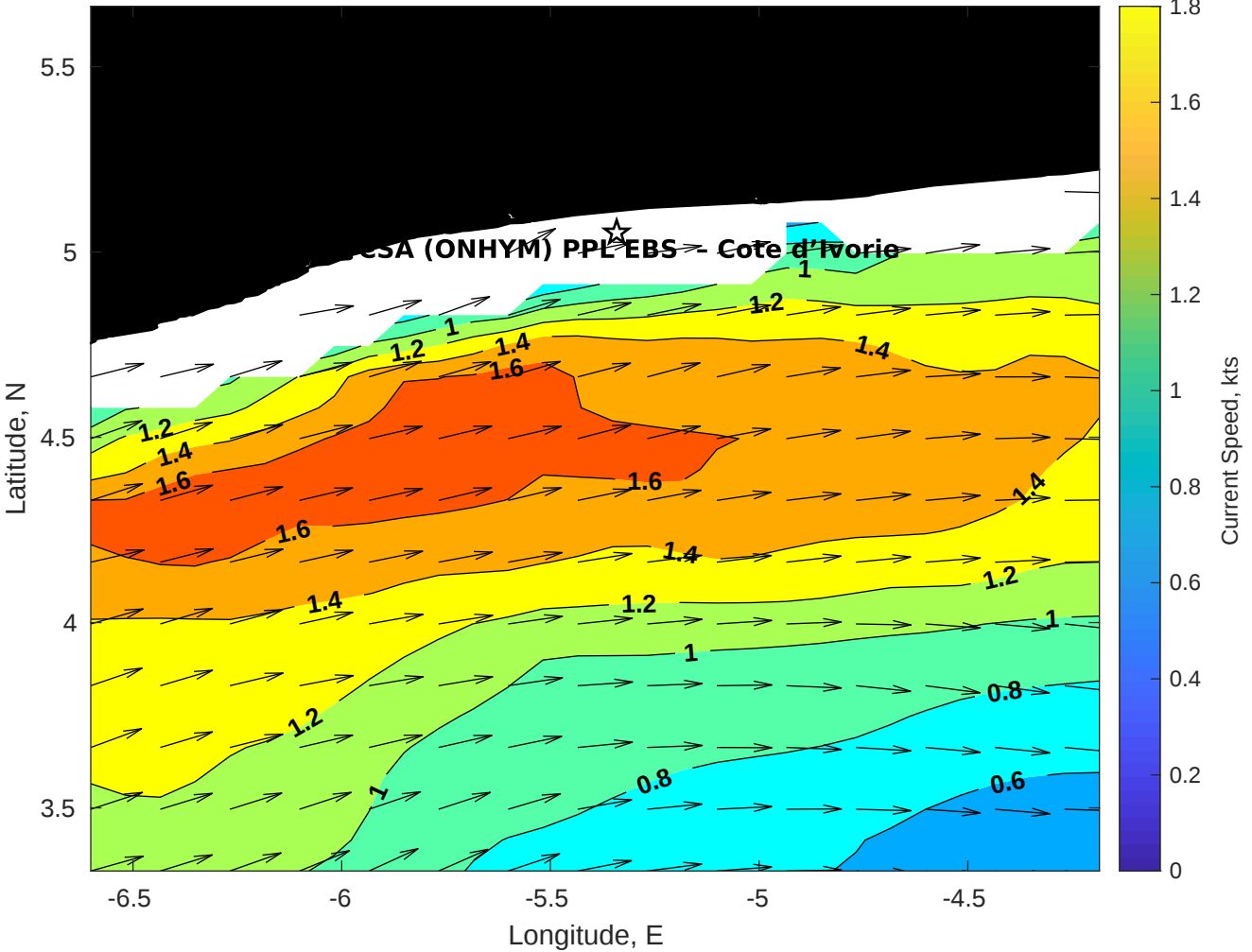
Surface Currents for CSA (ONHYM) PPL EBS - Cote d'Ivoire at 16-Jan-2026 00:00:00
