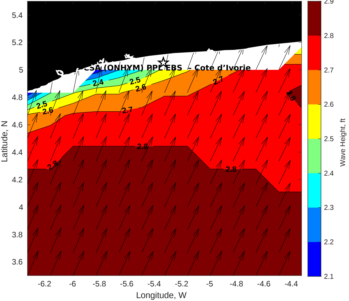
GFS Wave Height (ft) for CSA (ONHYM) PPL EBS - Cote d'Ivoire at 17-Jan-2026 09:00:00
