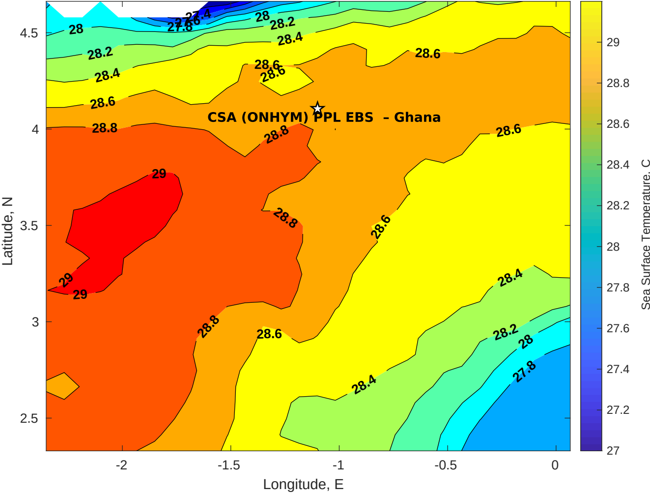
SST for CSA (ONHYM) PPL EBS - Ghana at 16-Jan-2026 00:00:00
