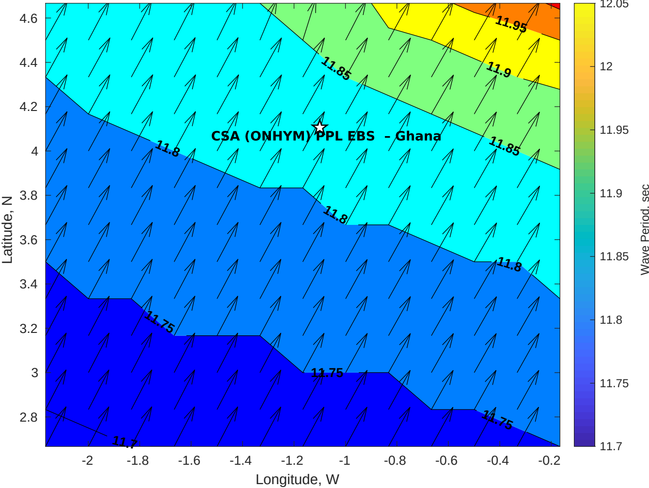
GFS Wave Period (sec) for CSA (ONHYM) PPL EBS - Ghana at 17-Jan-2026 09:00:00
