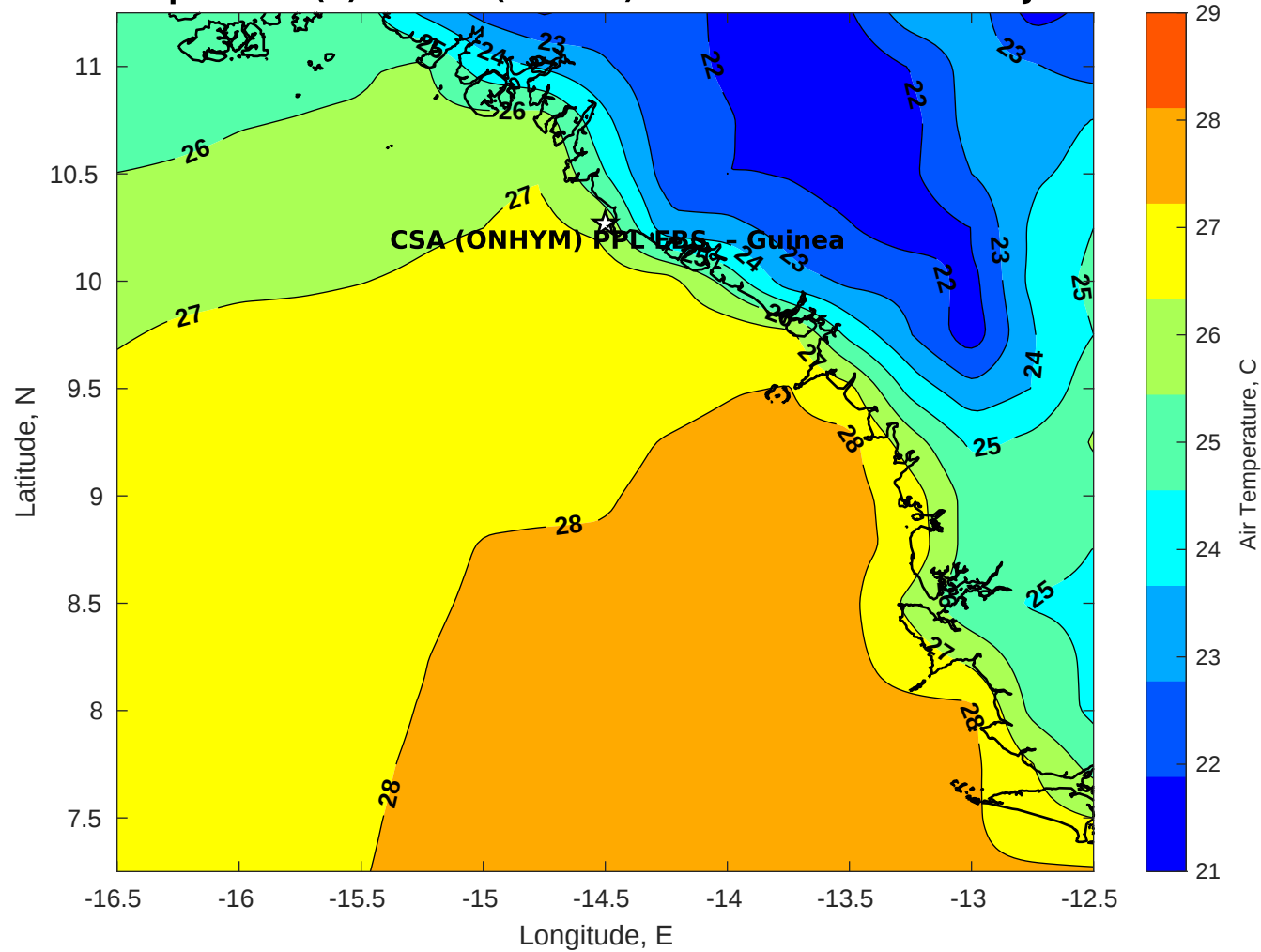
Air Temperature (C) for CSA (ONHYM) PPL EBS - Guinea at 17-Jan-2026
