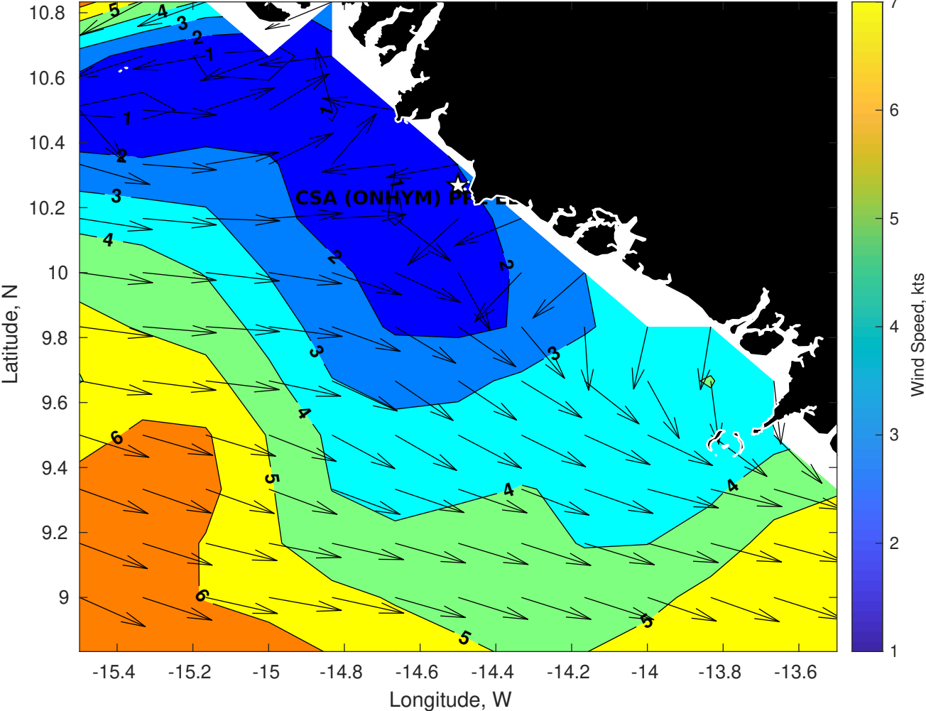
GFS Winds (kts) for CSA (ONHYM) PPL EBS - Guinea at 17-Jan-2026 09:00:00
