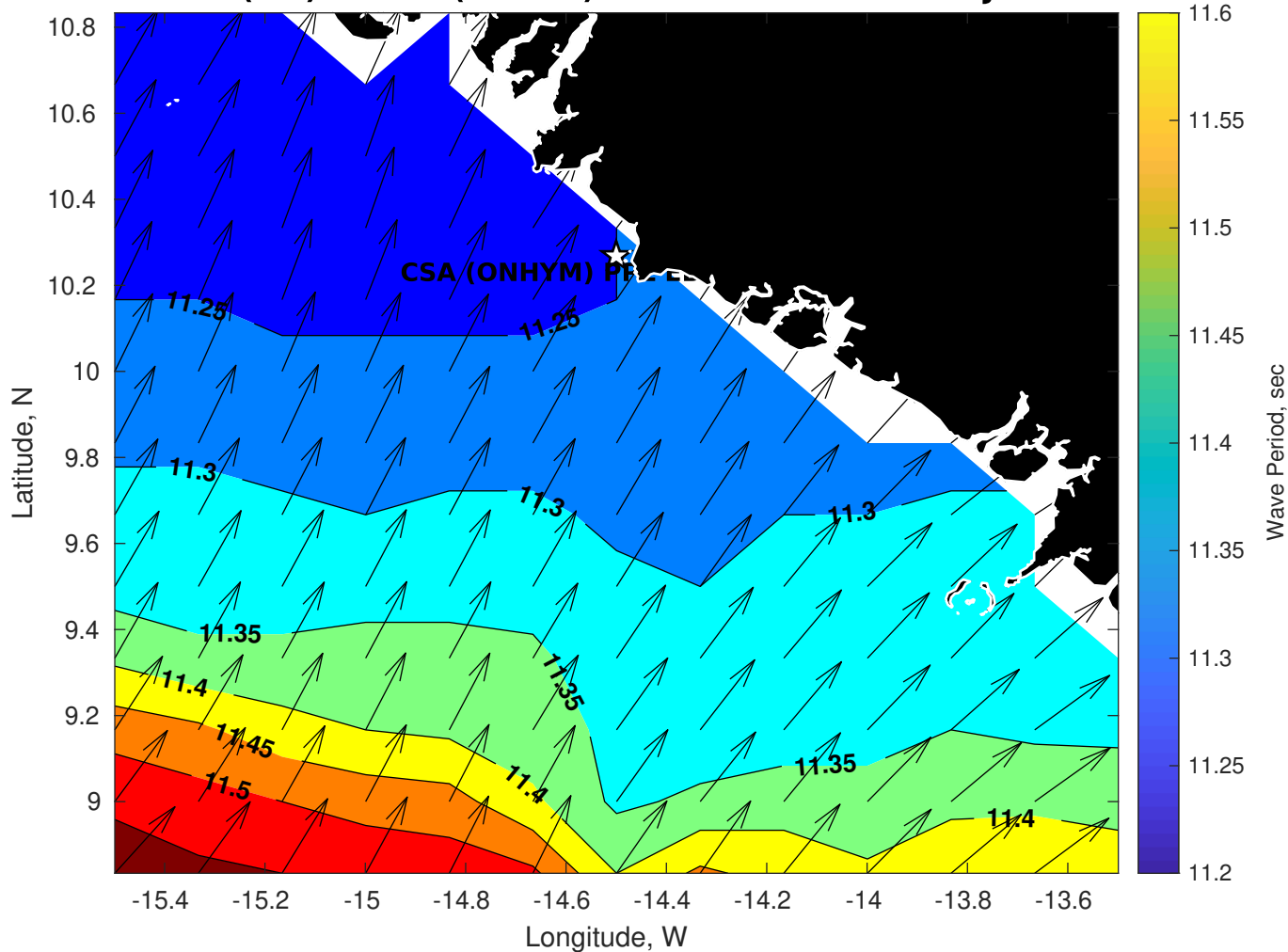
GFS Wave Period (sec) for CSA (ONHYM) PPL EBS - Guinea at 17-Jan-2026 09:00:00
