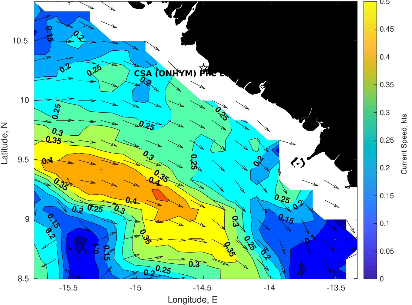
Surface Currents for CSA (ONHYM) PPL EBS - Guinea at 16-Jan-2026 00:00:00
