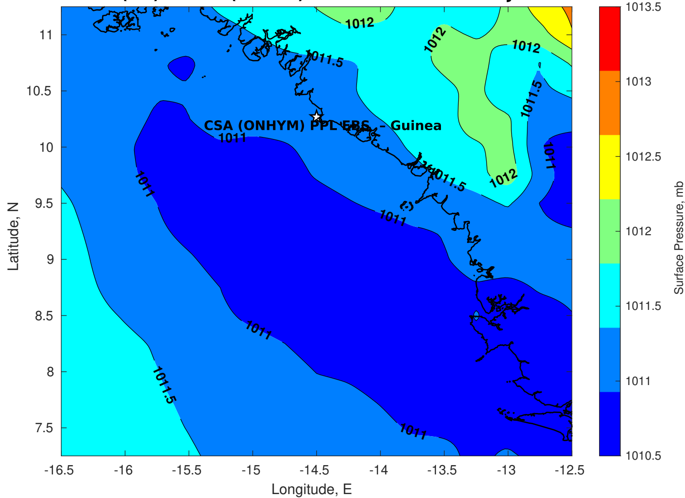
Surface Pressure (mb) for CSA (ONHYM) PPL EBS - Guinea at 18-Jan-2026 00:00:00
