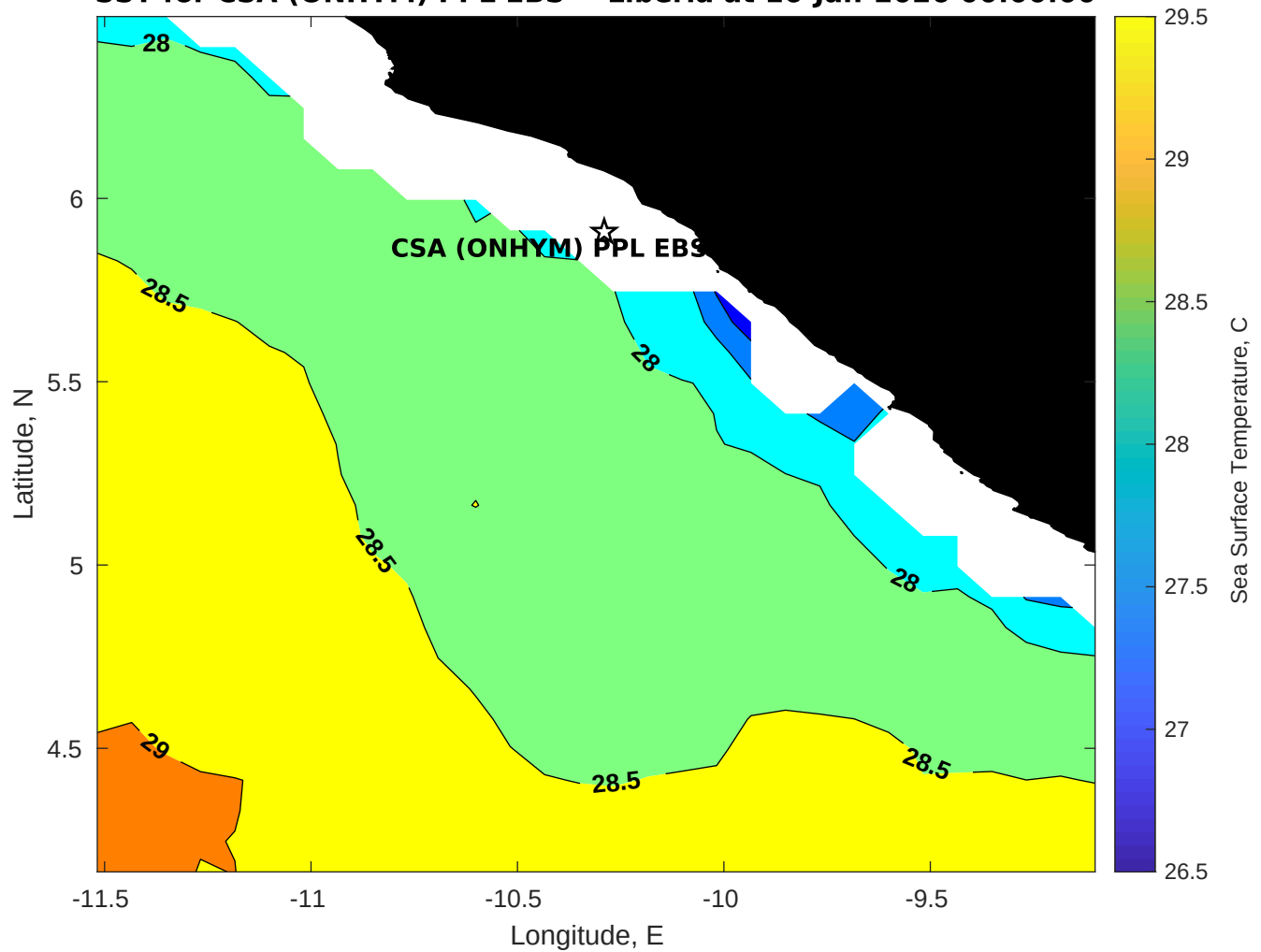
SST for CSA (ONHYM) PPL EBS - Liberia at 16-Jan-2026 00:00:00
