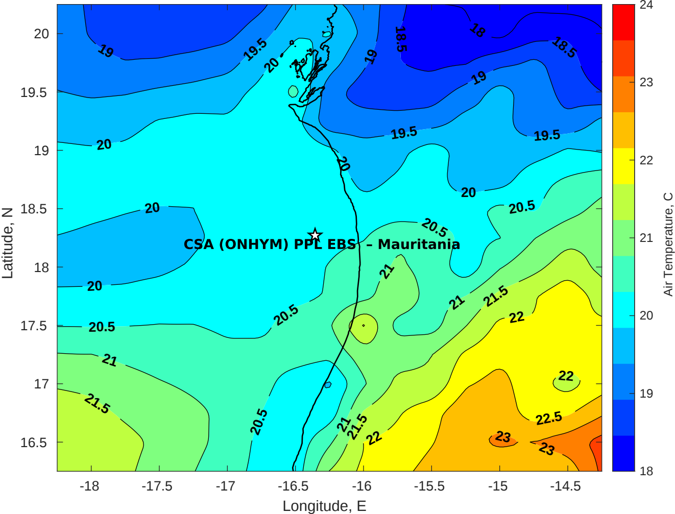
Air Temperature (C) for CSA (ONHYM) PPL EBS - Mauritania at 17-Jan-2026
