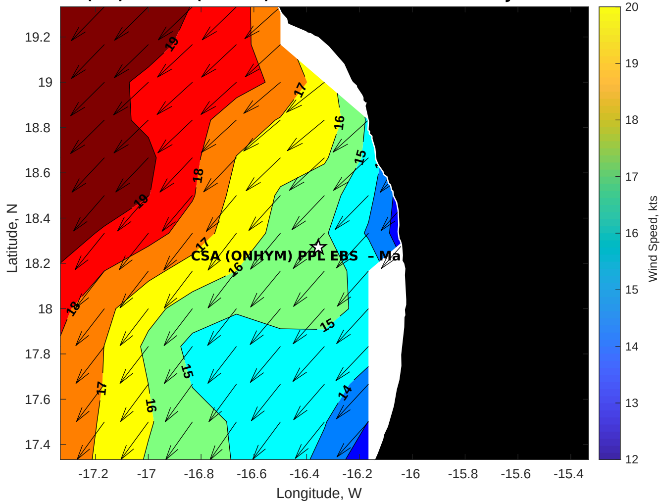
GFS Winds (kts) for CSA (ONHYM) PPL EBS - Mauritania at 17-Jan-2026 09:00:00
