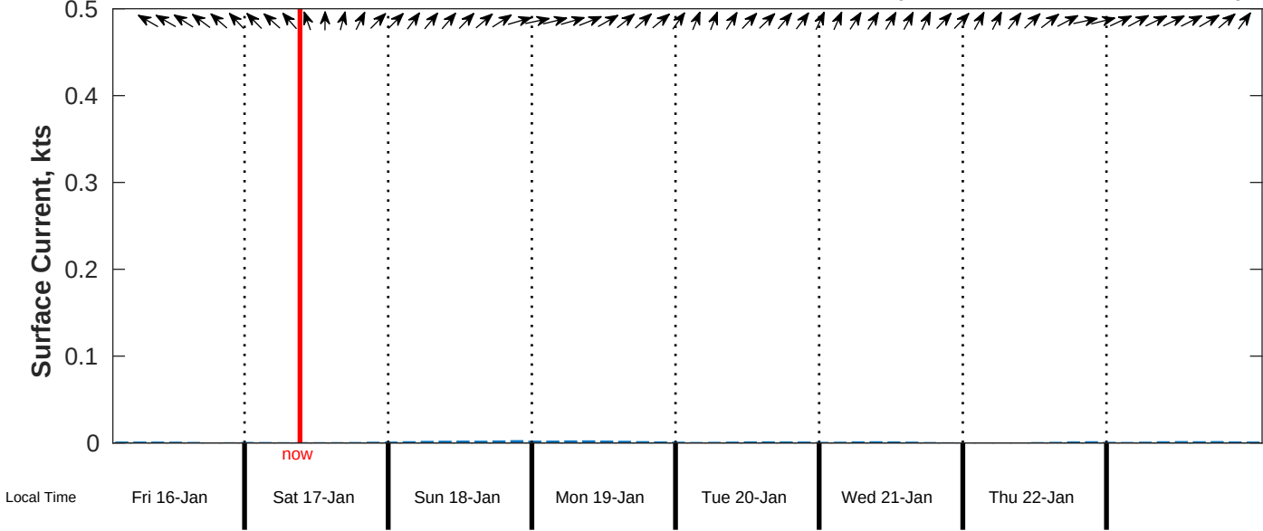
Surface Current Forecast for CSA (ONHYM) PPL EBS - Mauritania from 16-Jan-2026 00:00:00 to 24-Jan-2026 00:00:00
