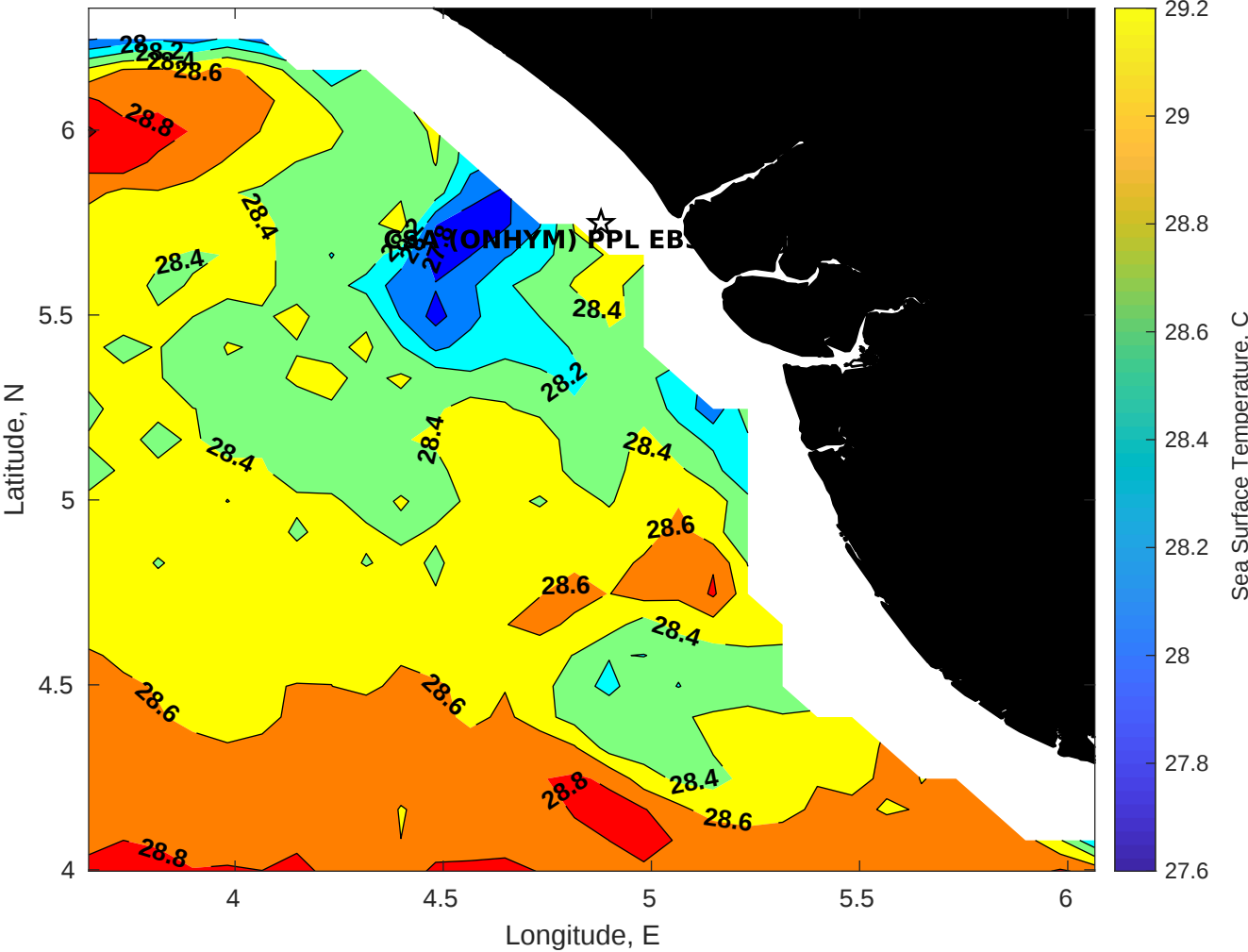
SST for CSA (ONHYM) PPL EBS - Nigeria at 16-Jan-2026 00:00:00
