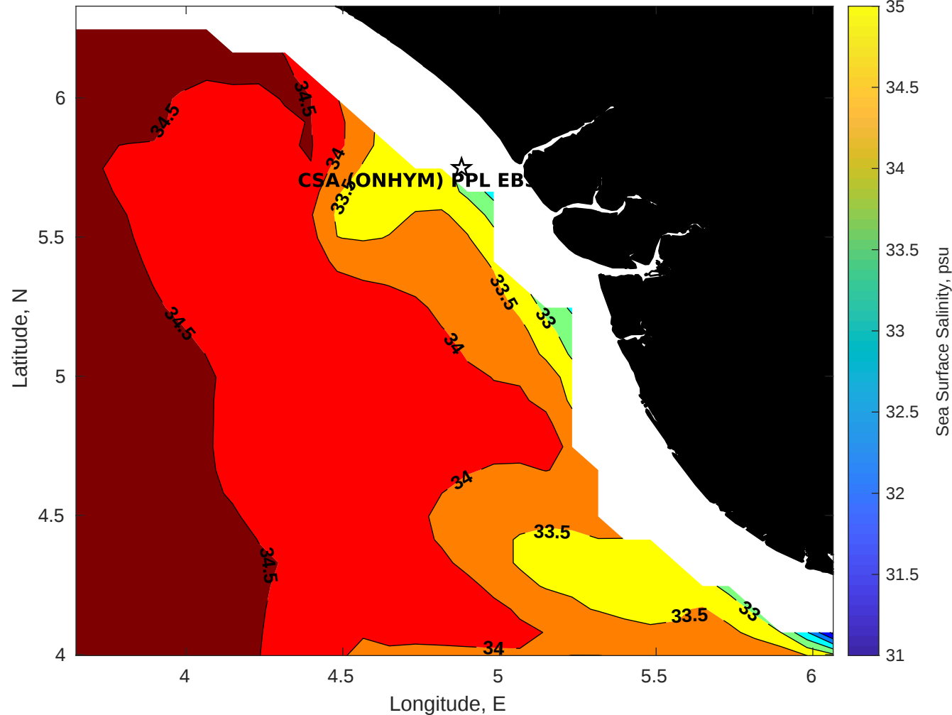
Surface Salinity for CSA (ONHYM) PPL EBS - Nigeria at 16-Jan-2026 00:00:00
