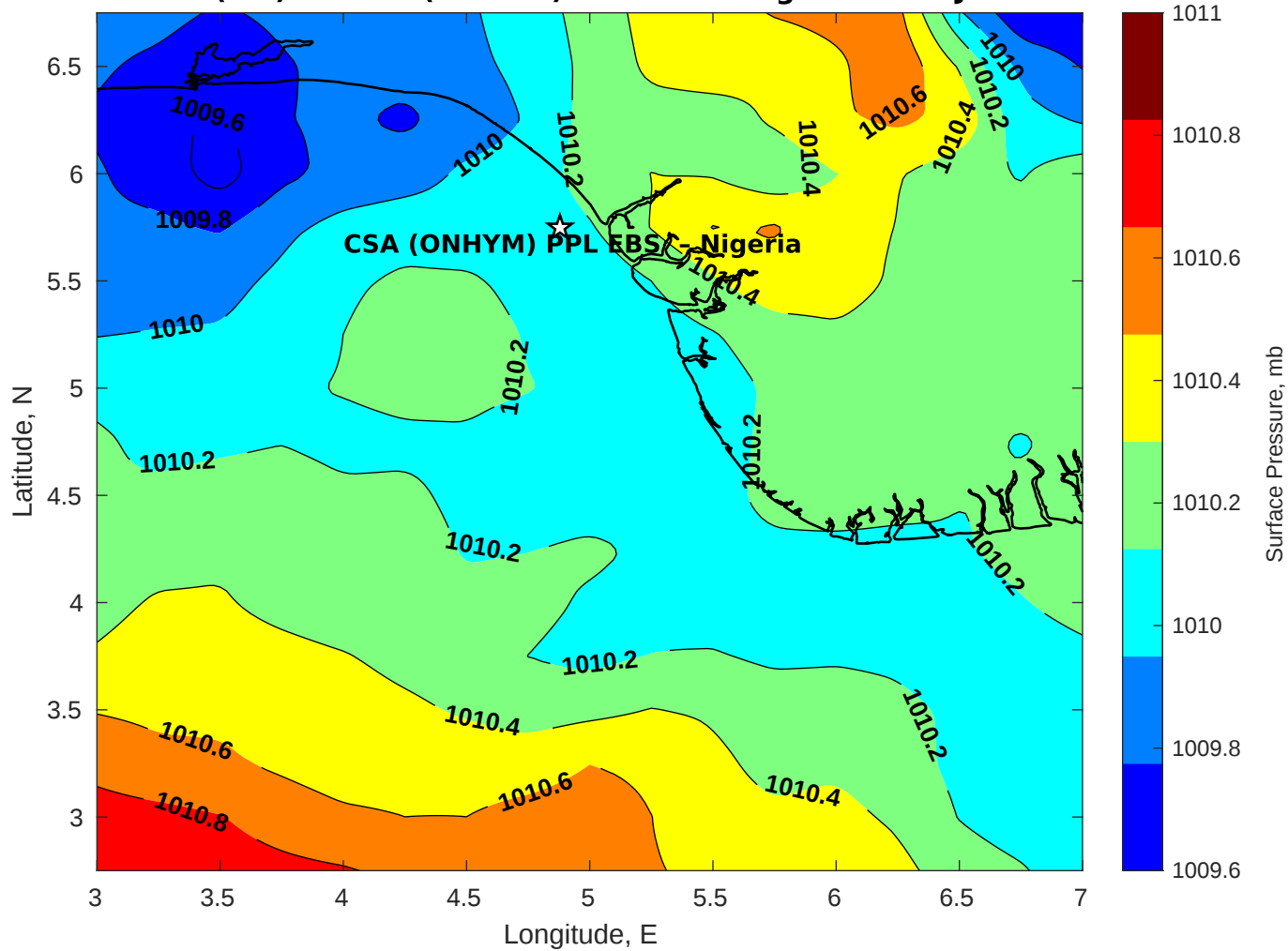
Surface Pressure (mb) for CSA (ONHYM) PPL EBS - Nigeria at 17-Jan-2026 00:00:00
