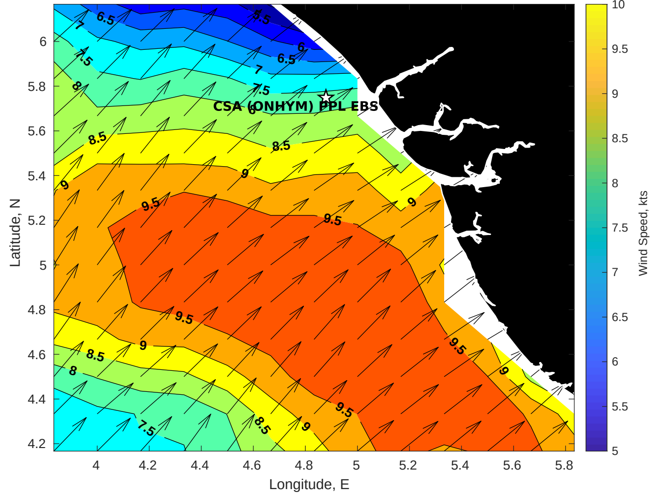
GFS Winds (kts) for CSA (ONHYM) PPL EBS - Nigeria at 17-Jan-2026 09:00:00
