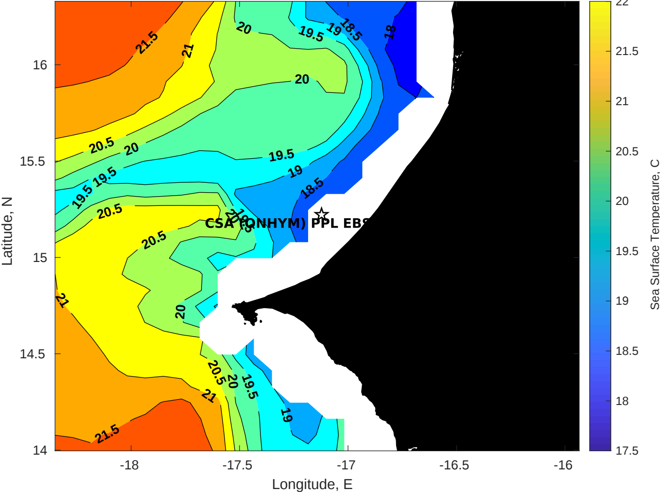
SST for CSA (ONHYM) PPL EBS - Senegal at 16-Jan-2026 00:00:00
