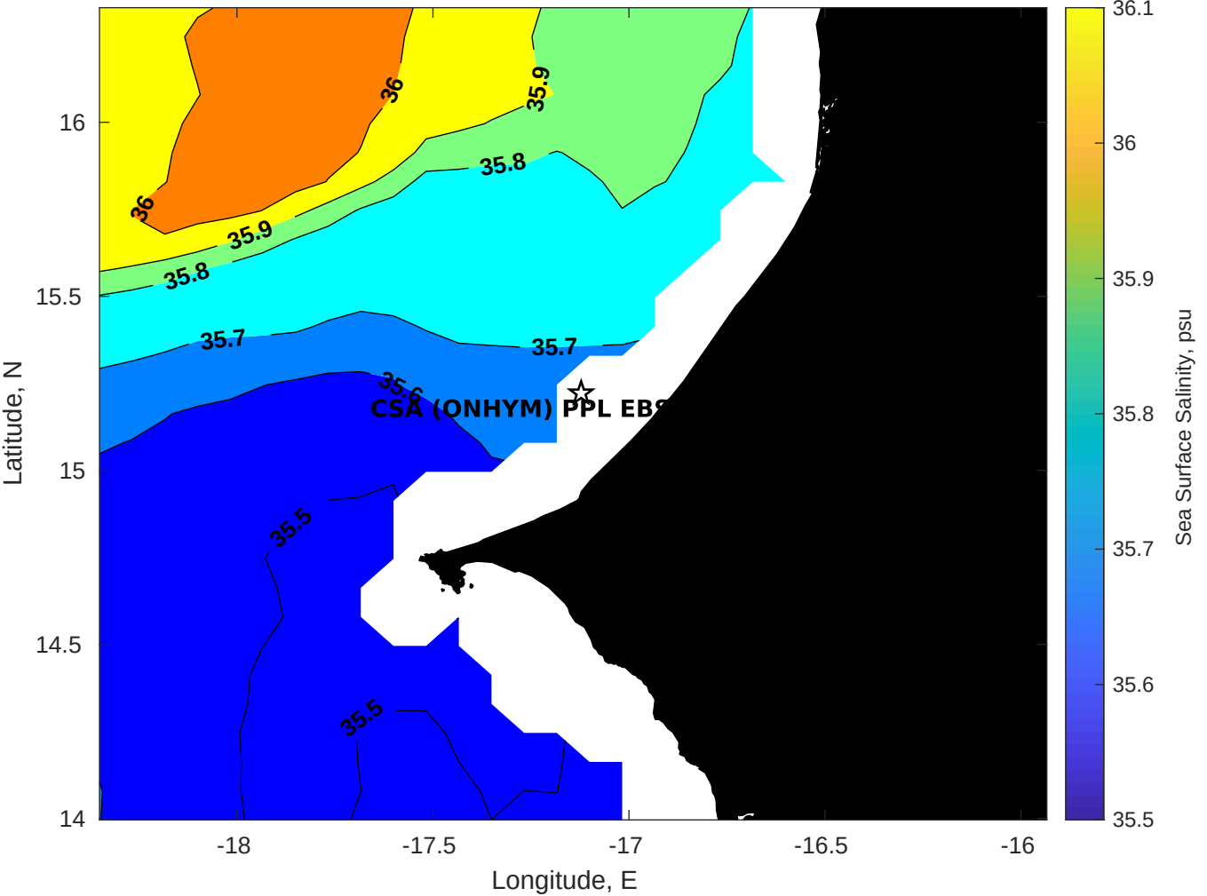
Surface Salinity for CSA (ONHYM) PPL EBS - Senegal at 16-Jan-2026 00:00:00
