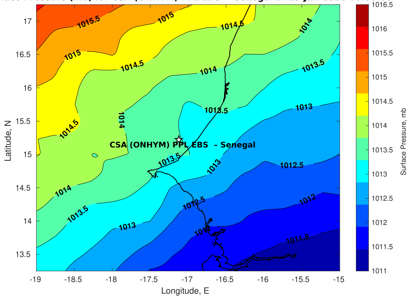
Surface Pressure (mb) for CSA (ONHYM) PPL EBS - Senegal at 19-Jan-2026 00:00:00
