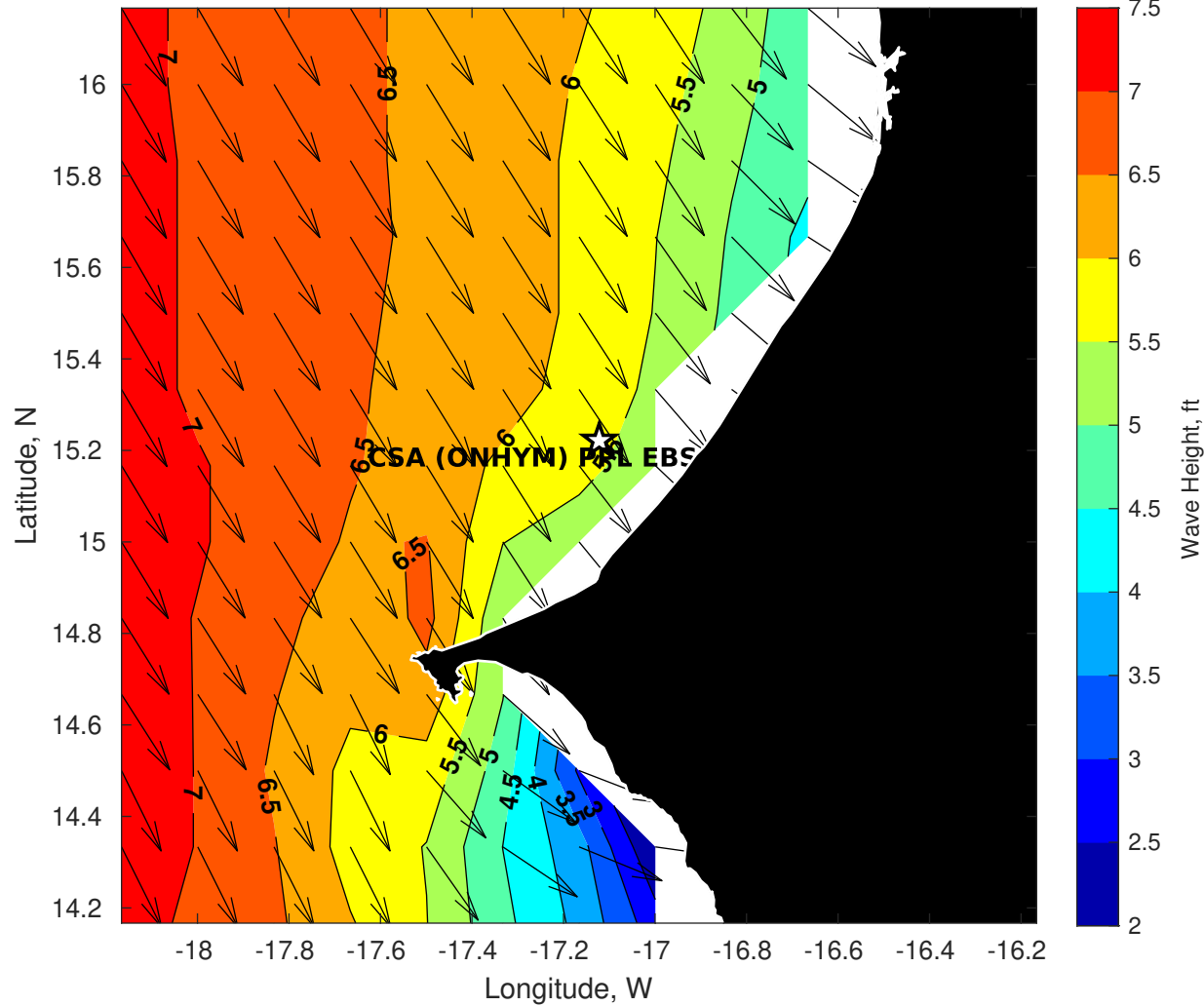
GFS Wave Height (ft) for CSA (ONHYM) PPL EBS - Senegal at 17-Jan-2026 09:00:00
