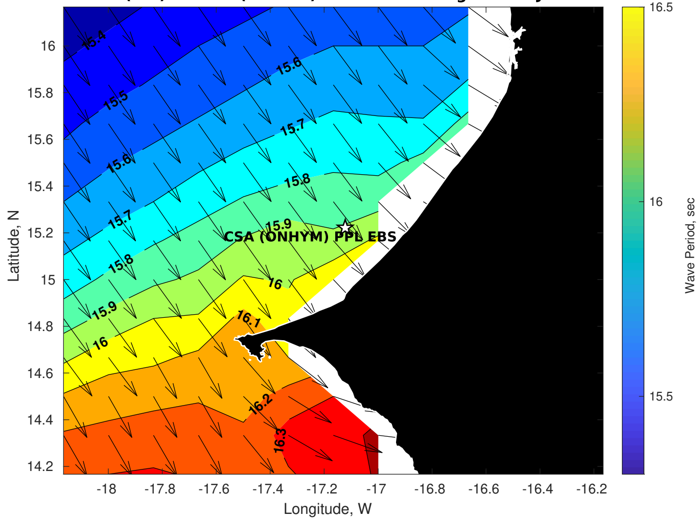
GFS Wave Period (sec) for CSA (ONHYM) PPL EBS - Senegal at 17-Jan-2026 09:00:00
