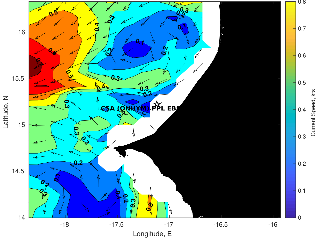
Surface Currents for CSA (ONHYM) PPL EBS - Senegal at 16-Jan-2026 00:00:00
