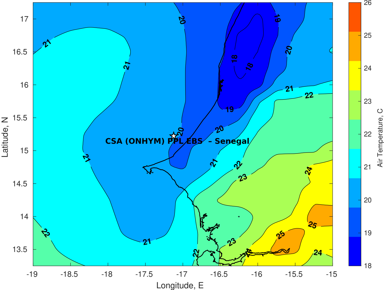
Air Temperature (C) for CSA (ONHYM) PPL EBS - Senegal at 17-Jan-2026
