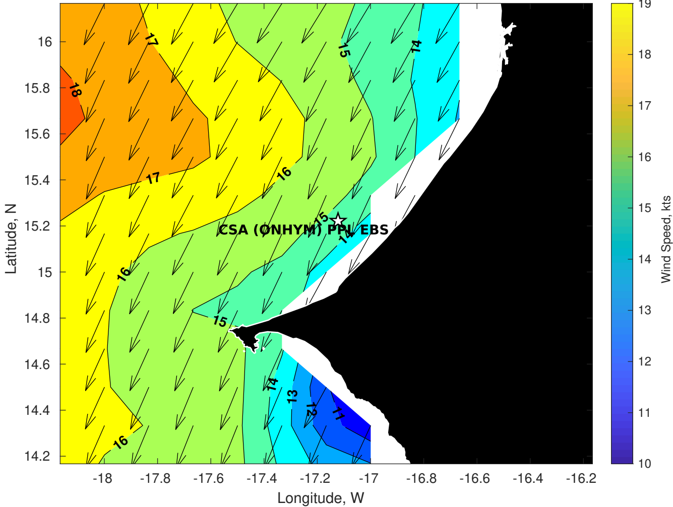
GFS Winds (kts) for CSA (ONHYM) PPL EBS - Senegal at 17-Jan-2026 09:00:00
