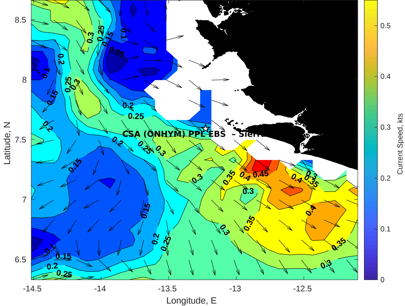
Surface Currents for CSA (ONHYM) PPL EBS - Sierra Leone at 16-Jan-2026 00:00:00
