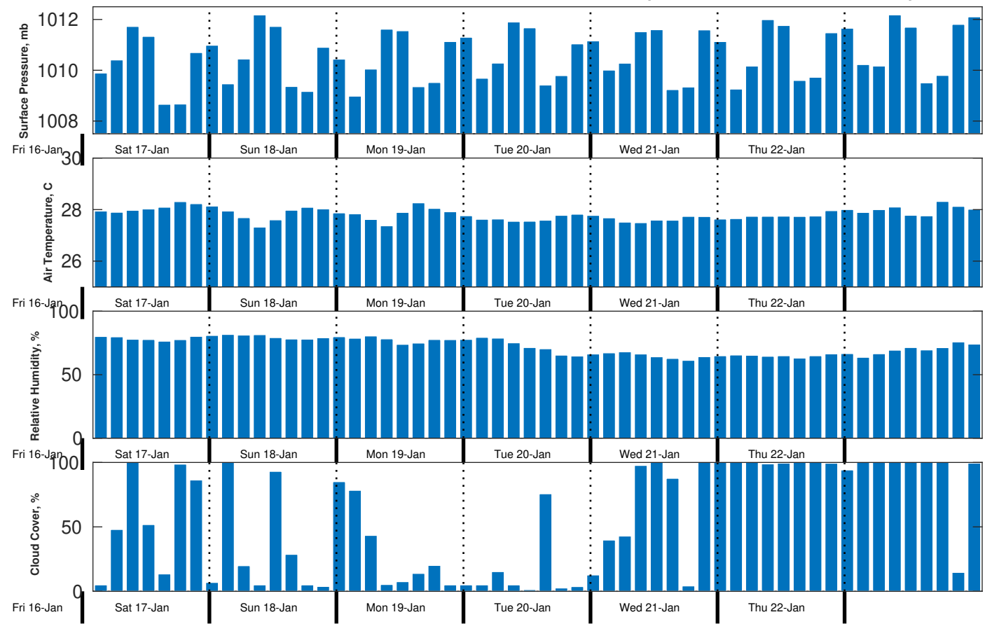
Met Forecast for CSA (ONHYM) PPL EBS - Sierra Leone from 17-Jan-2026 00:00:00 to 24-Jan-2026 00:00:00
