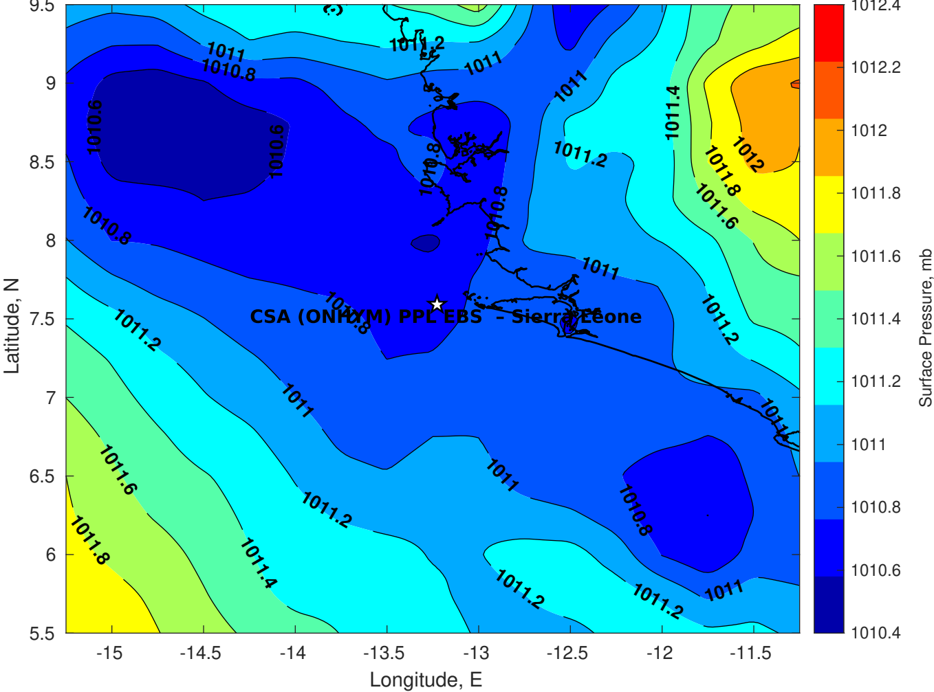
Surface Pressure (mb) for CSA (ONHYM) PPL EBS - Sierra Leone at 17-Jan-2026 00:00:00
