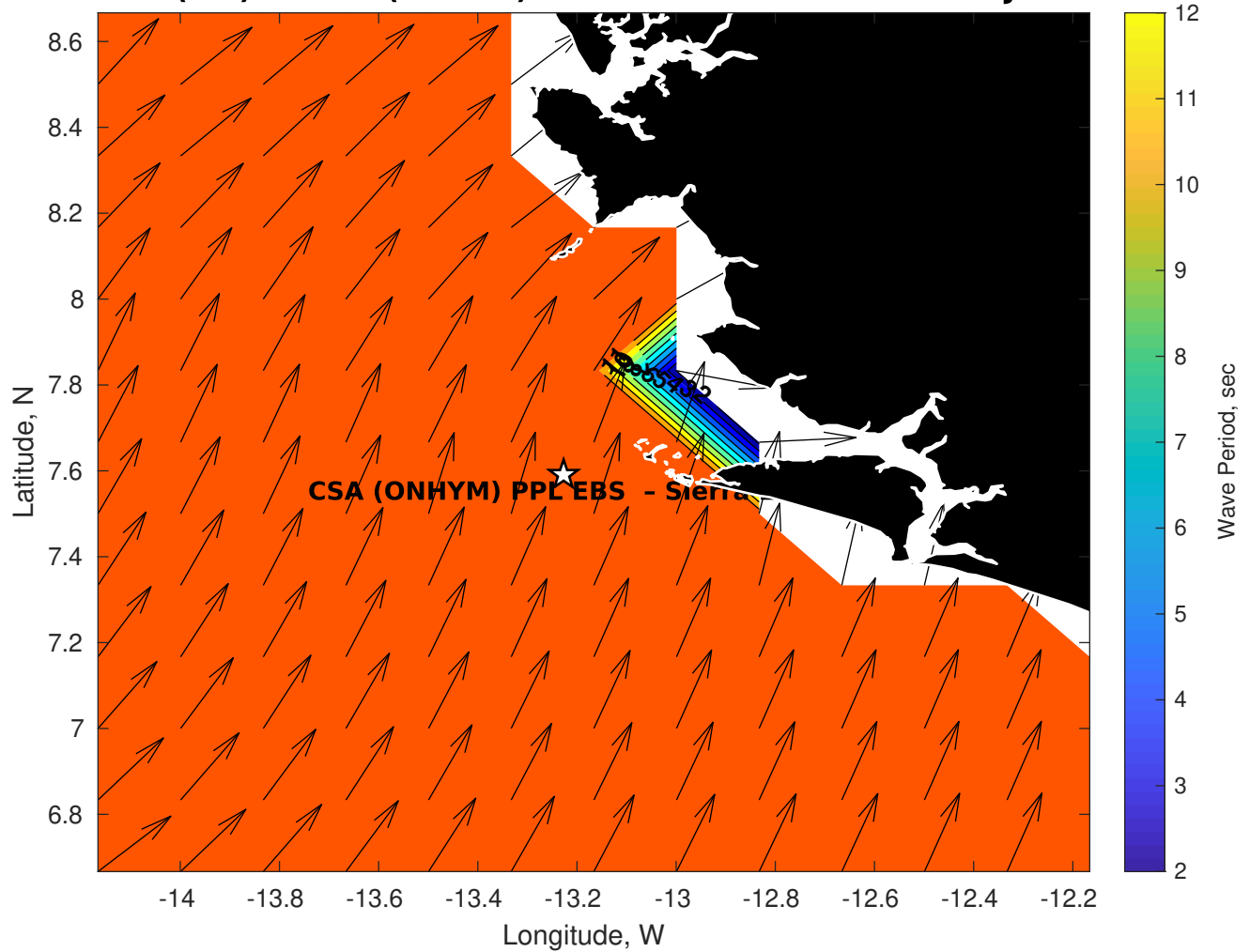
GFS Wave Period (sec) for CSA (ONHYM) PPL EBS - Sierra Leone at 17-Jan-2026 09:00:00
