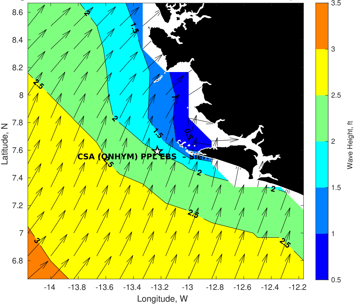
GFS Wave Height (ft) for CSA (ONHYM) PPL EBS - Sierra Leone at 17-Jan-2026 09:00:00
