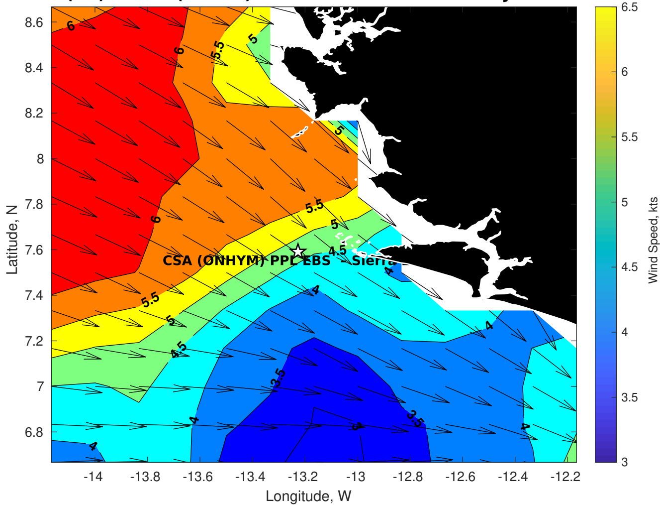
GFS Winds (kts) for CSA (ONHYM) PPL EBS - Sierra Leone at 17-Jan-2026 09:00:00
