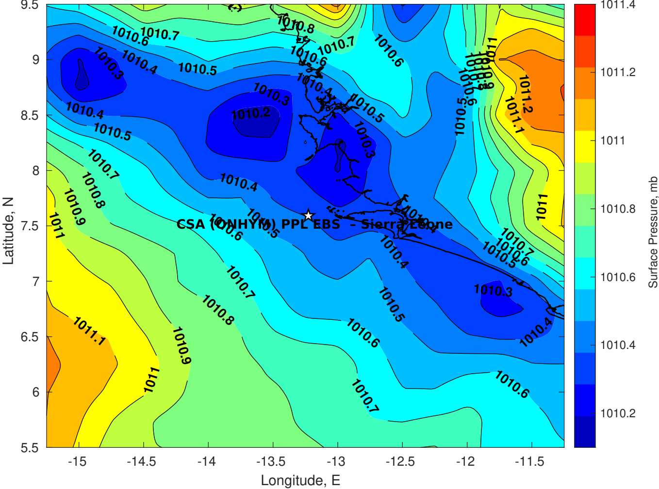
Surface Pressure (mb) for CSA (ONHYM) PPL EBS - Sierra Leone at 19-Jan-2026 00:00:00
