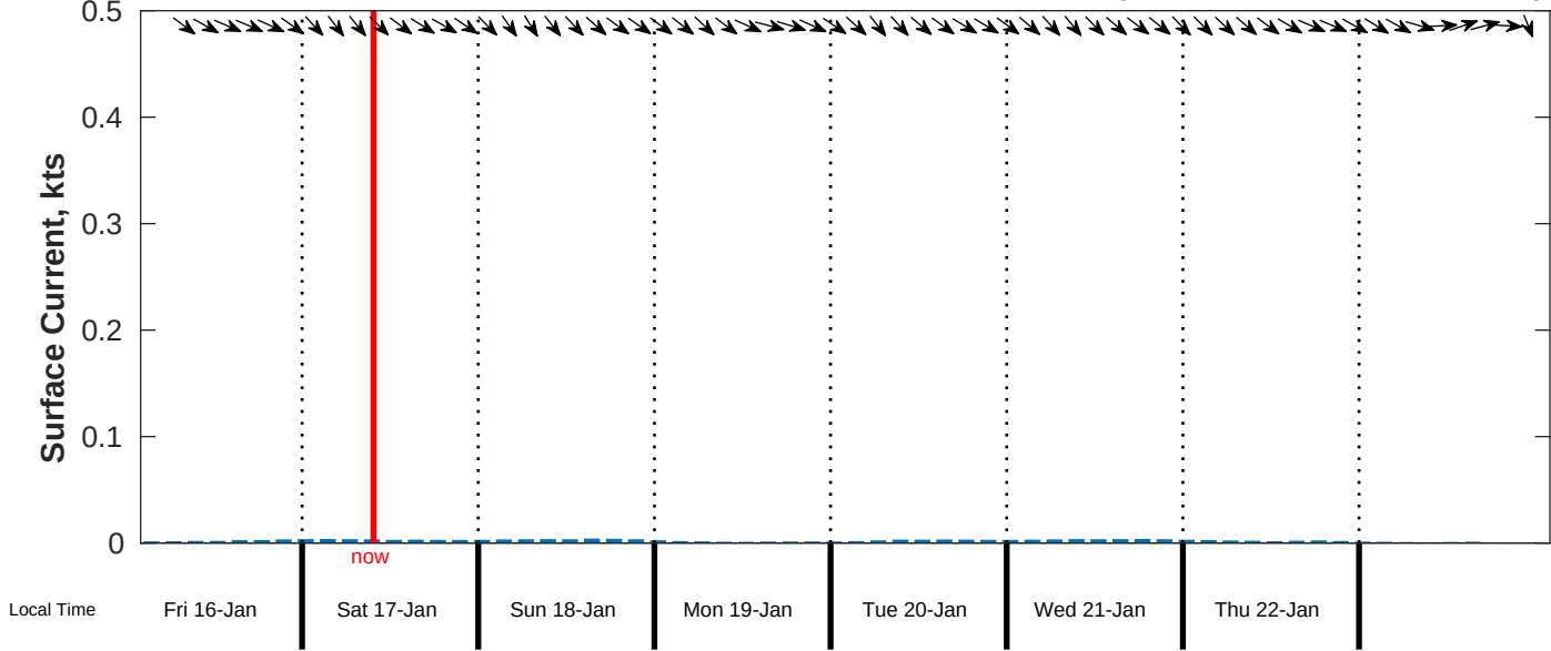
Surface Current Forecast for CSA (ONHYM) PPL EBS - Sierra Leone from 16-Jan-2026 00:00:00 to 24-Jan-2026 00:00:00
