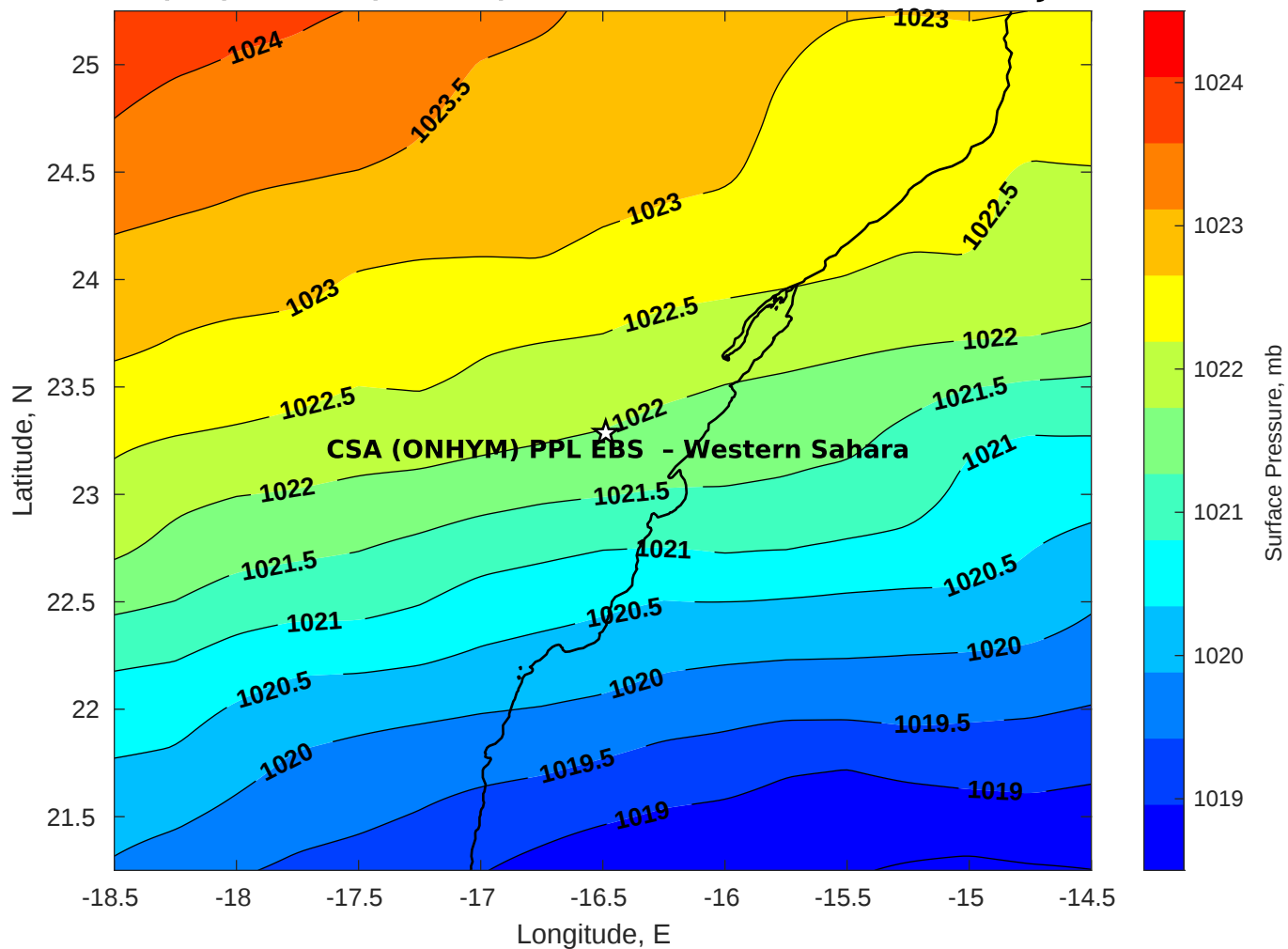
Surface Pressure (mb) for CSA (ONHYM) PPL EBS - Western Sahara at 17-Jan-2026 00:00:00
