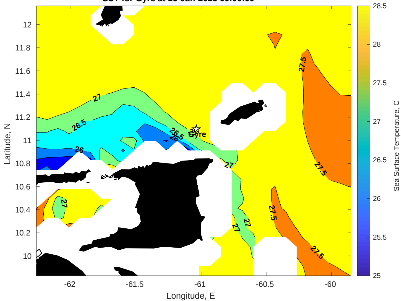
SST for Gyre at 16-Jan-2026 00:00:00
