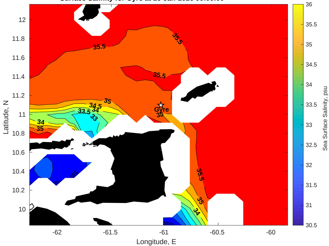
Surface Salinity for Gyre at 16-Jan-2026 00:00:00
