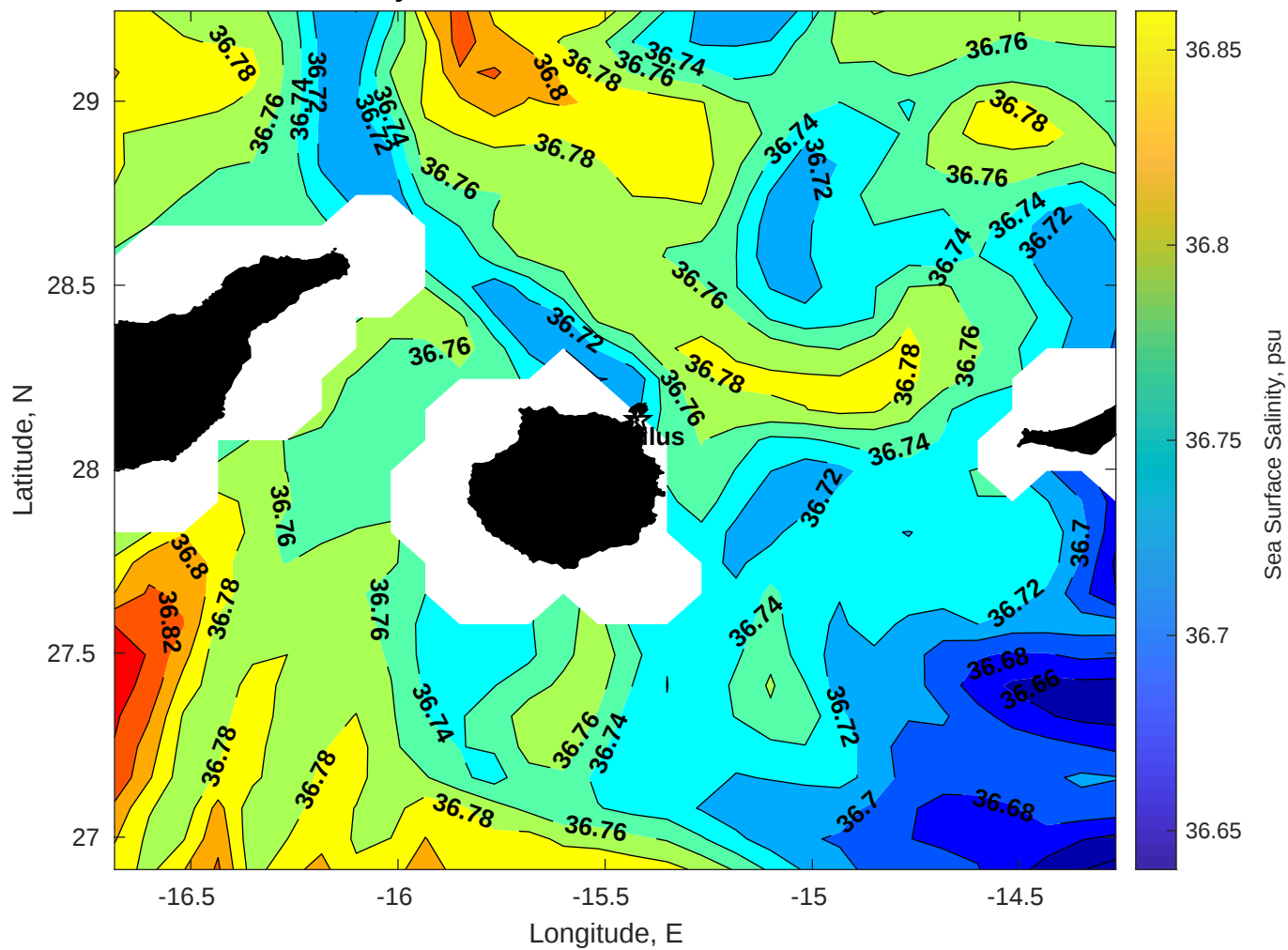
Surface Salinity for Nautilus at 16-Jan-2026 00:00:00
