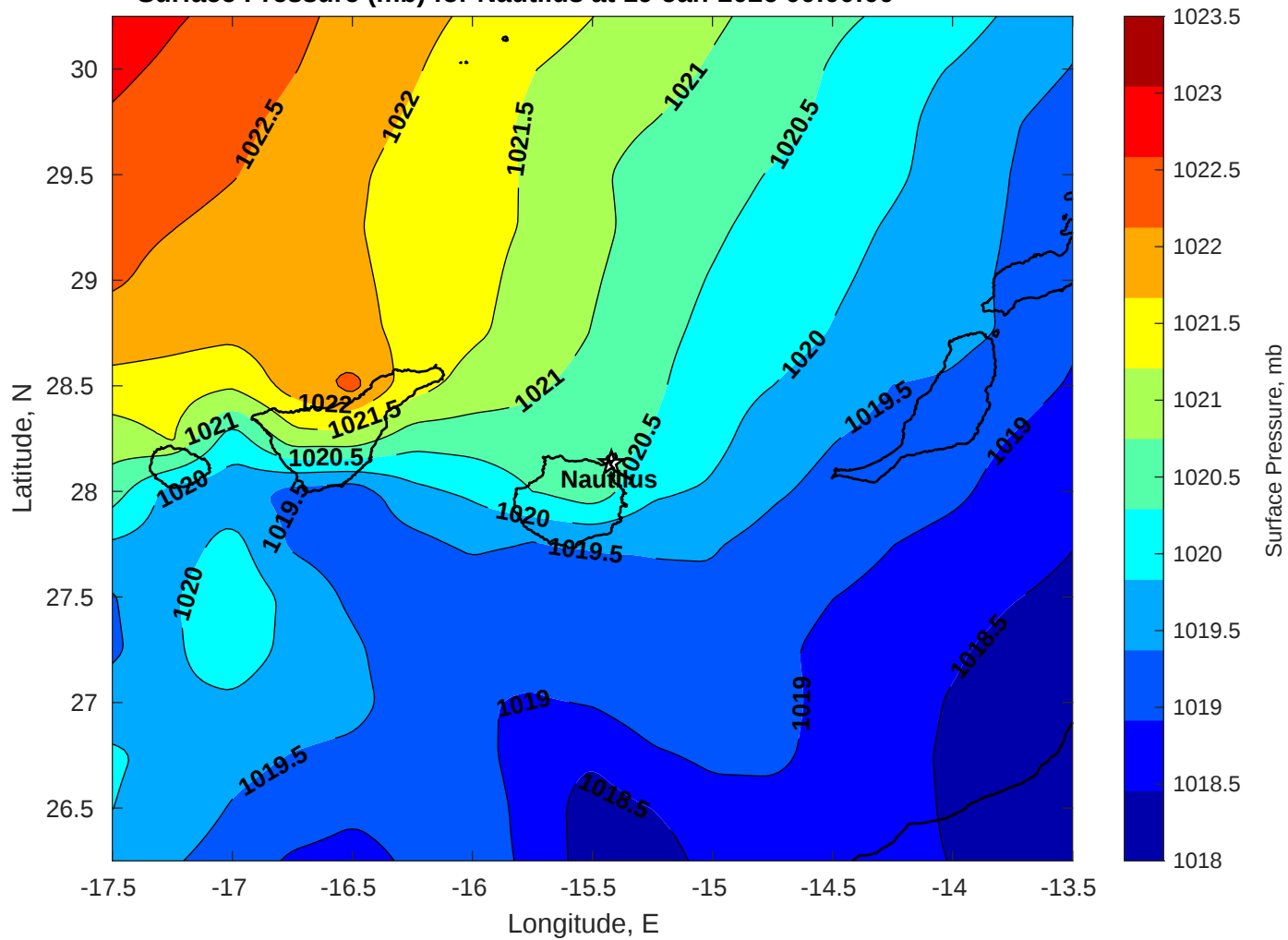
Surface Pressure (mb) for Nautilus at 19-Jan-2026 00:00:00
