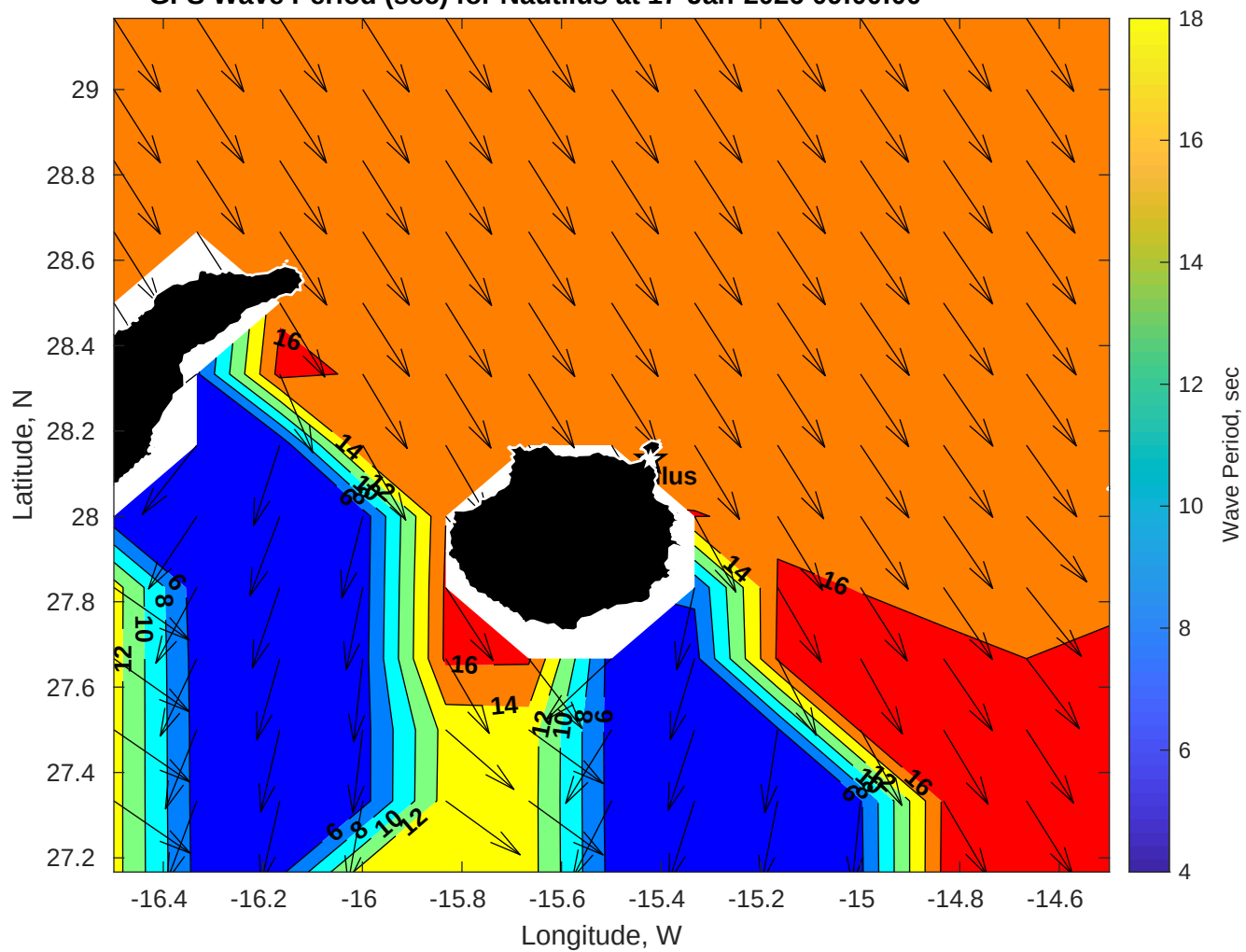
GFS Wave Period (sec) for Nautilus at 17-Jan-2026 09:00:00
