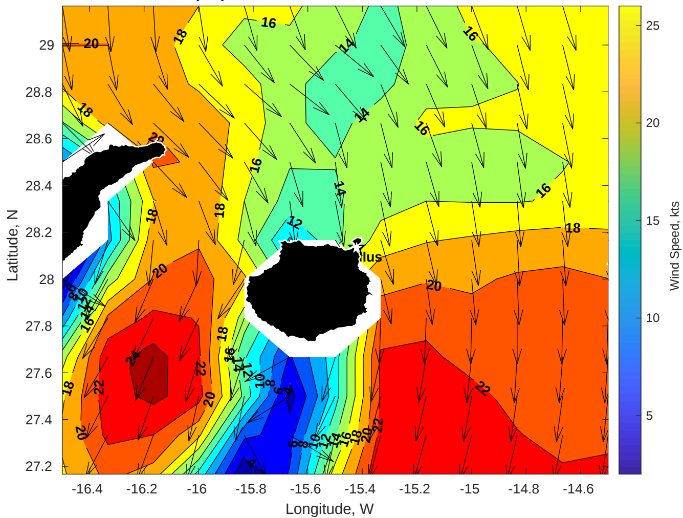
GFS Winds (kts) for Nautilus at 17-Jan-2026 09:00:00
