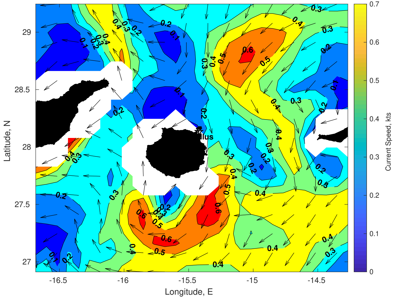
Surface Currents for Nautilus at 16-Jan-2026 00:00:00
