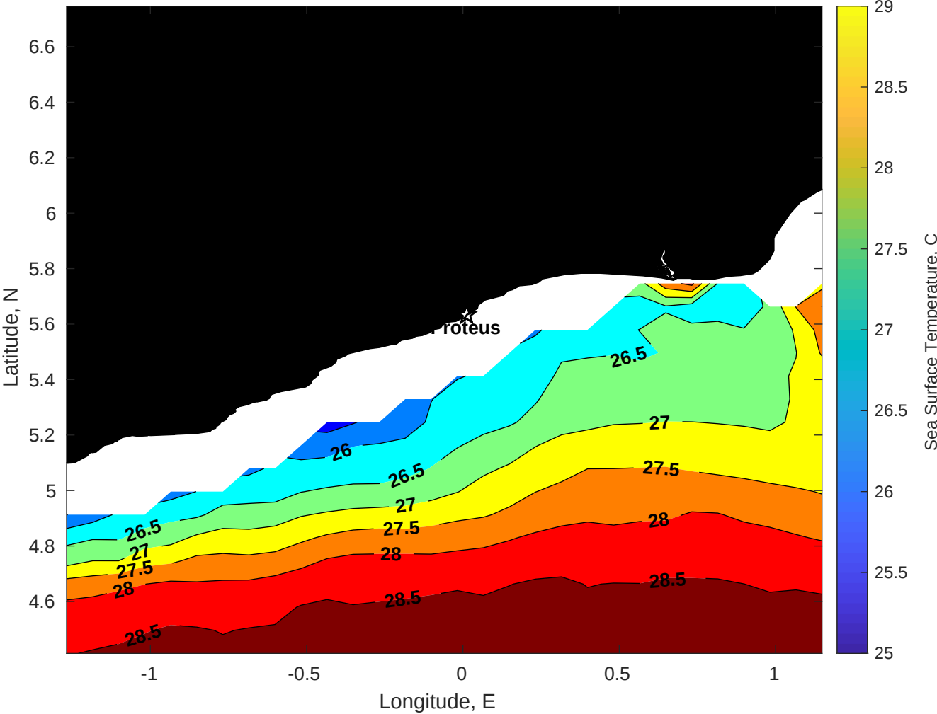
SST for Proteus at 16-Jan-2026 00:00:00
