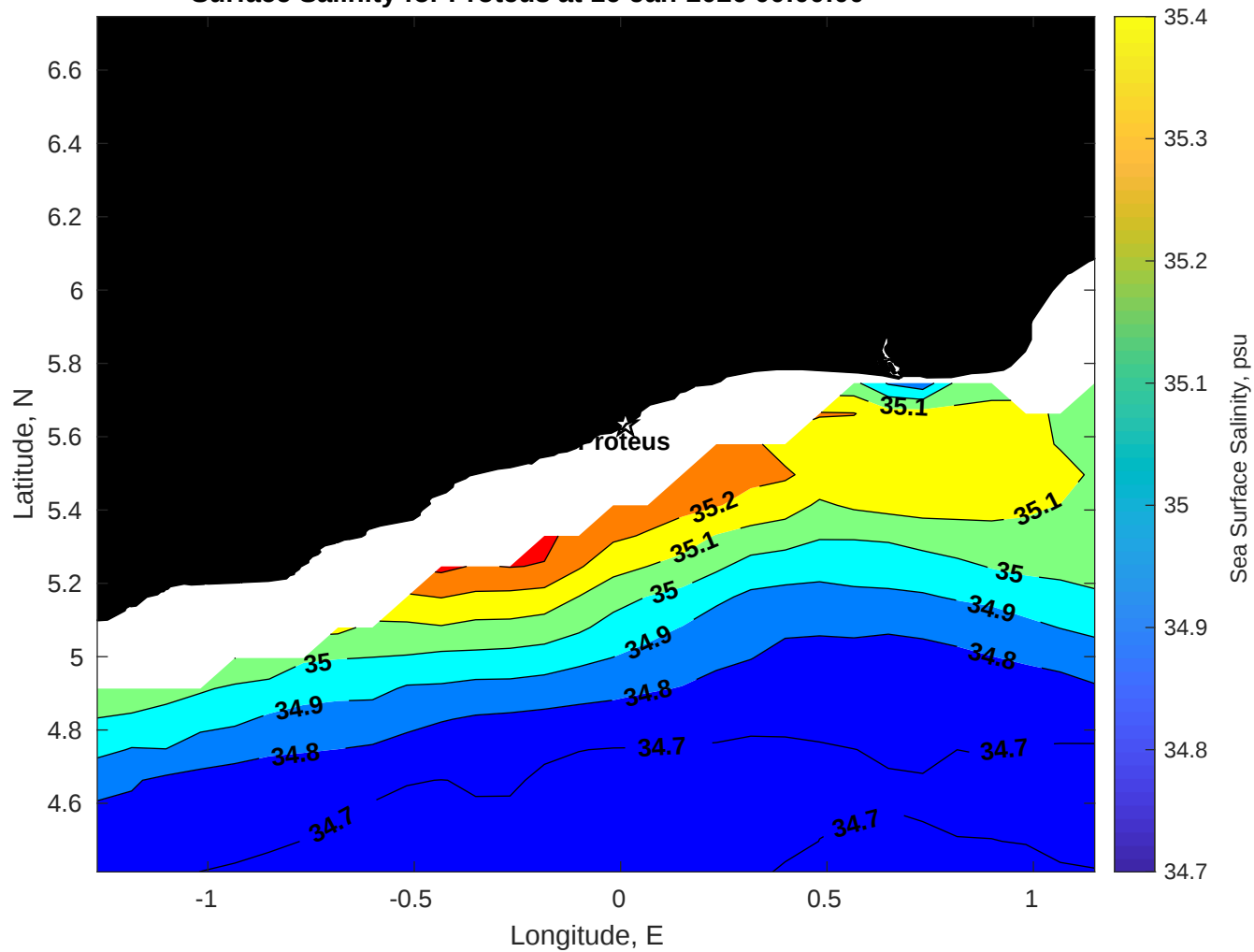
Surface Salinity for Proteus at 16-Jan-2026 00:00:00
