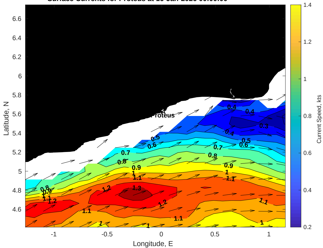
Surface Currents for Proteus at 16-Jan-2026 00:00:00
