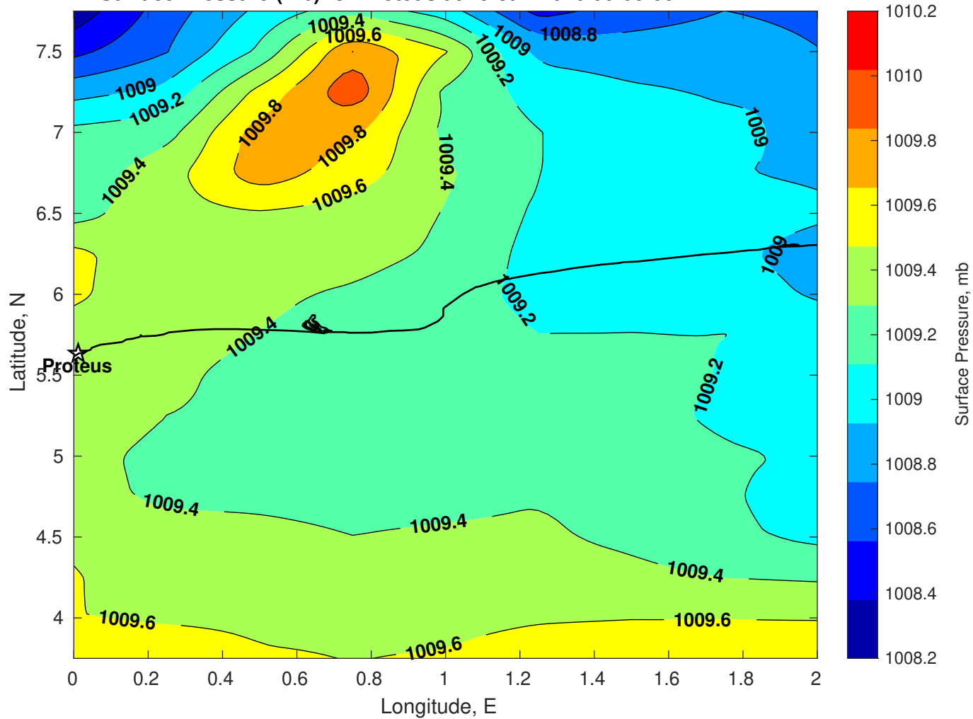
Surface Pressure (mb) for Proteus at 19-Jan-2026 00:00:00
