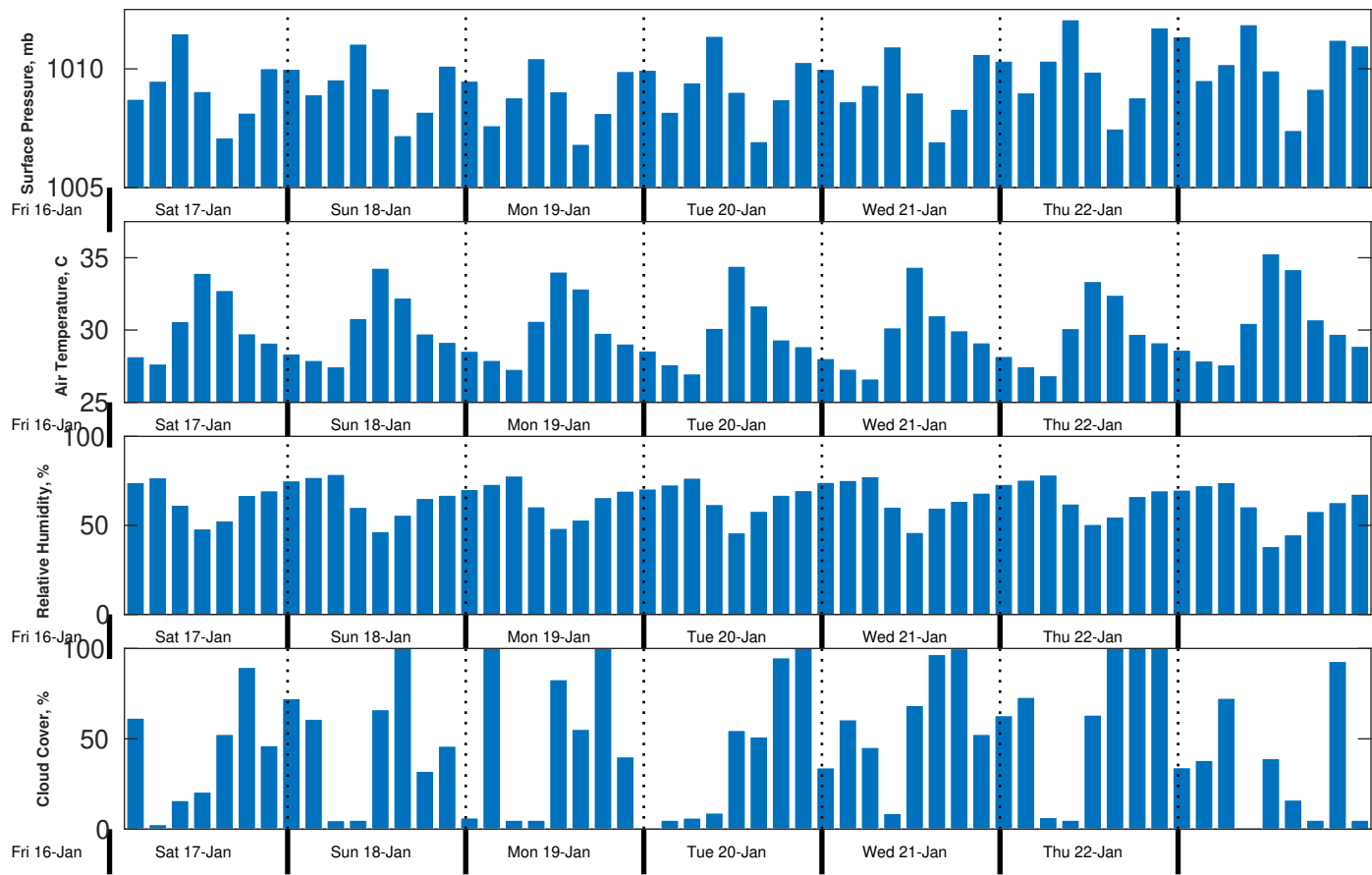
Met Forecast for Proteus from 17-Jan-2026 00:00:00 to 24-Jan-2026 00:00:00
