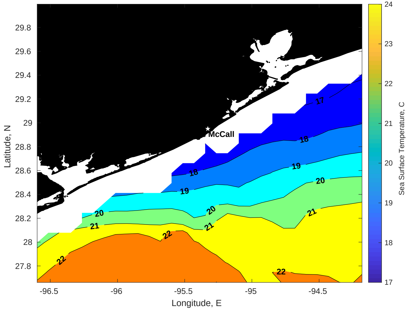
SST for Brooks McCall at 17-Jan-2026 00:00:00
