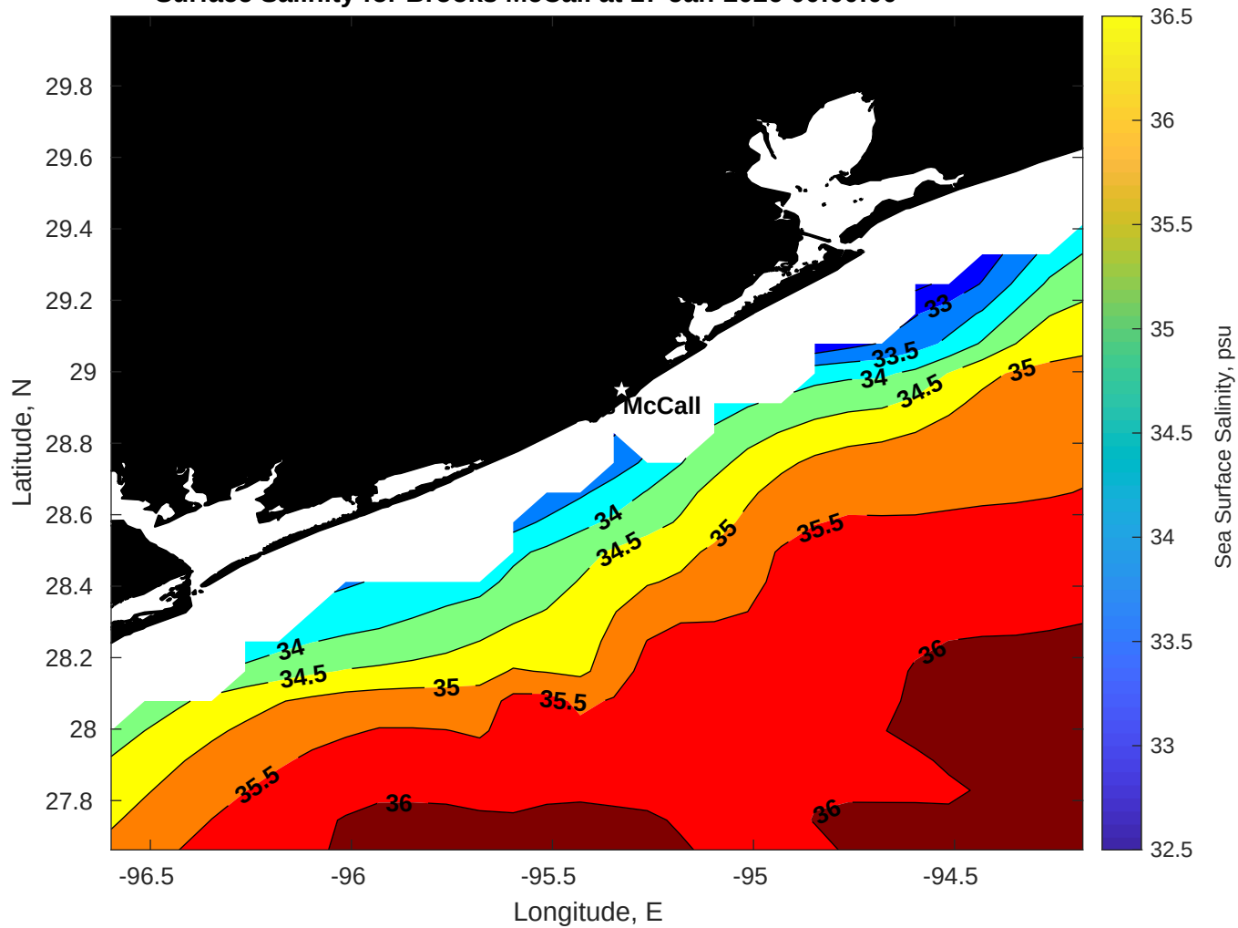
Surface Salinity for Brooks McCall at 17-Jan-2026 00:00:00
