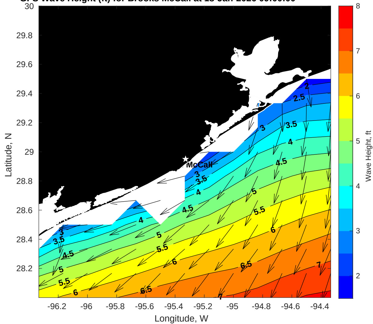
GFS Wave Height (ft) for Brooks McCall at 18-Jan-2026 09:00:00
