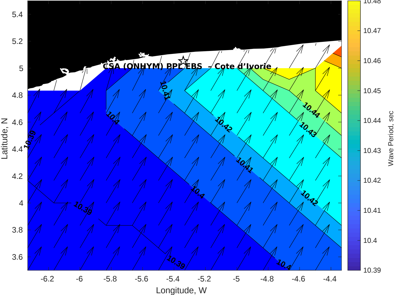
GFS Wave Period (sec) for CSA (ONHYM) PPL EBS - Cote d'Ivoire at 18-Jan-2026 09:00:00
