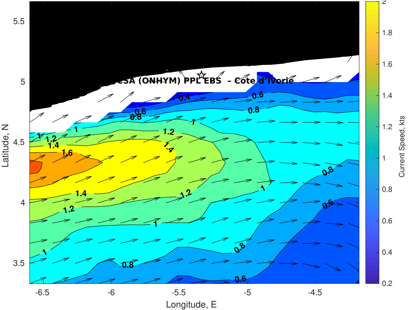
Surface Currents for CSA (ONHYM) PPL EBS - Cote d'Ivoire at 17-Jan-2026 00:00:00
