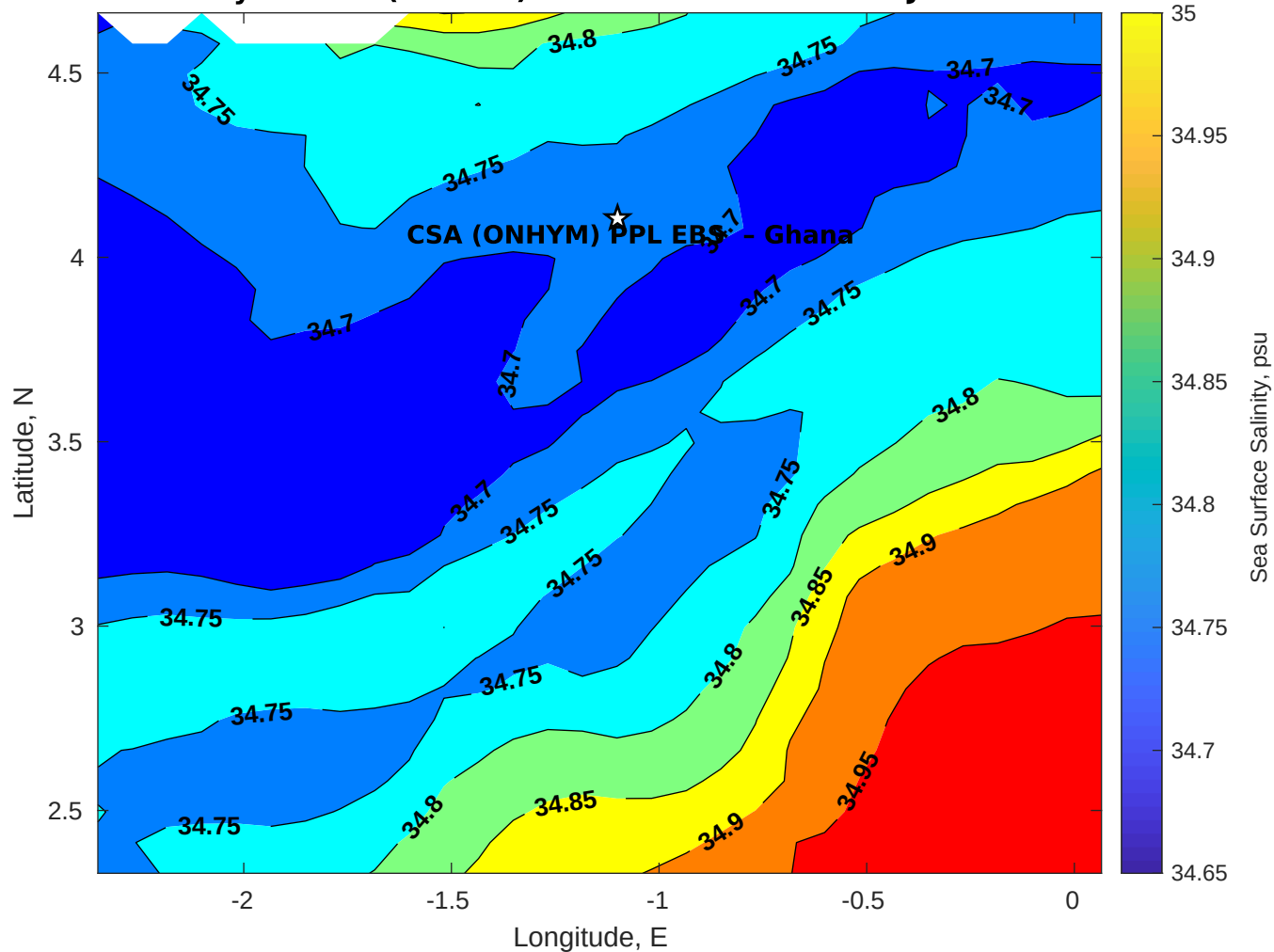
Surface Salinity for CSA (ONHYM) PPL EBS - Ghana at 17-Jan-2026 00:00:00
