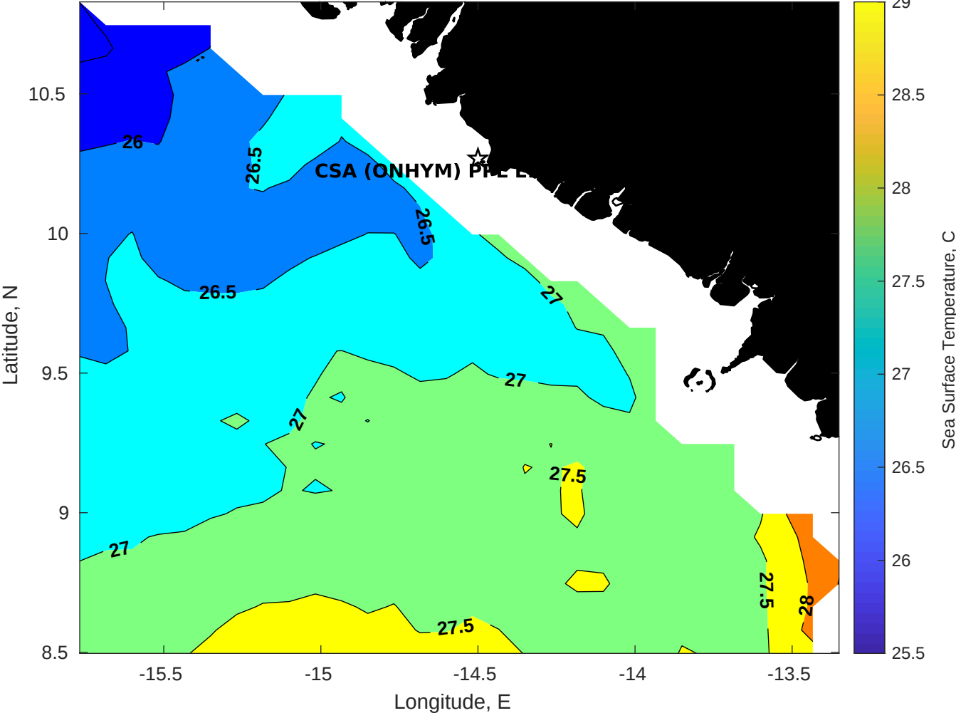
SST for CSA (ONHYM) PPL EBS - Guinea at 17-Jan-2026 00:00:00
