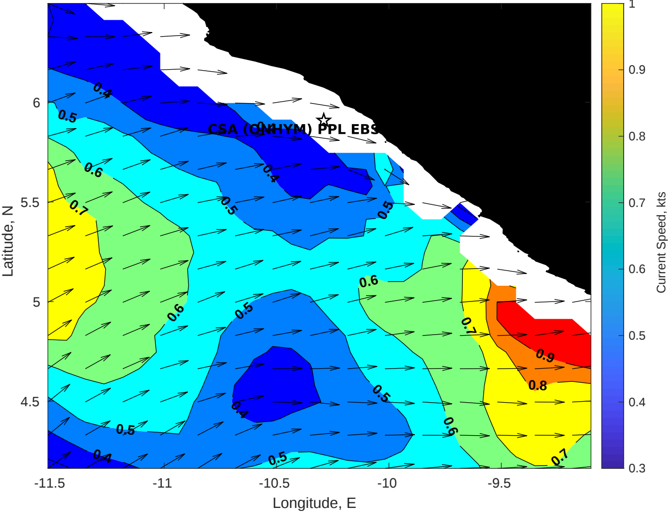
Surface Currents for CSA (ONHYM) PPL EBS - Liberia at 17-Jan-2026 00:00:00
