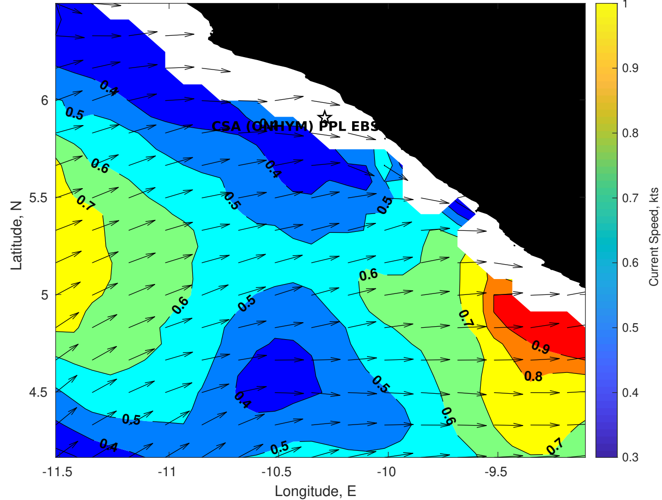
Surface Currents for CSA (ONHYM) PPL EBS - Liberia at 17-Jan-2026 00:00:00
