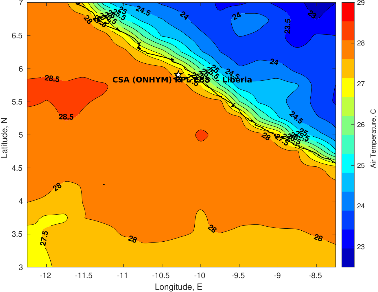
Air Temperature (C) for CSA (ONHYM) PPL EBS - Liberia at 18-Jan-2026
