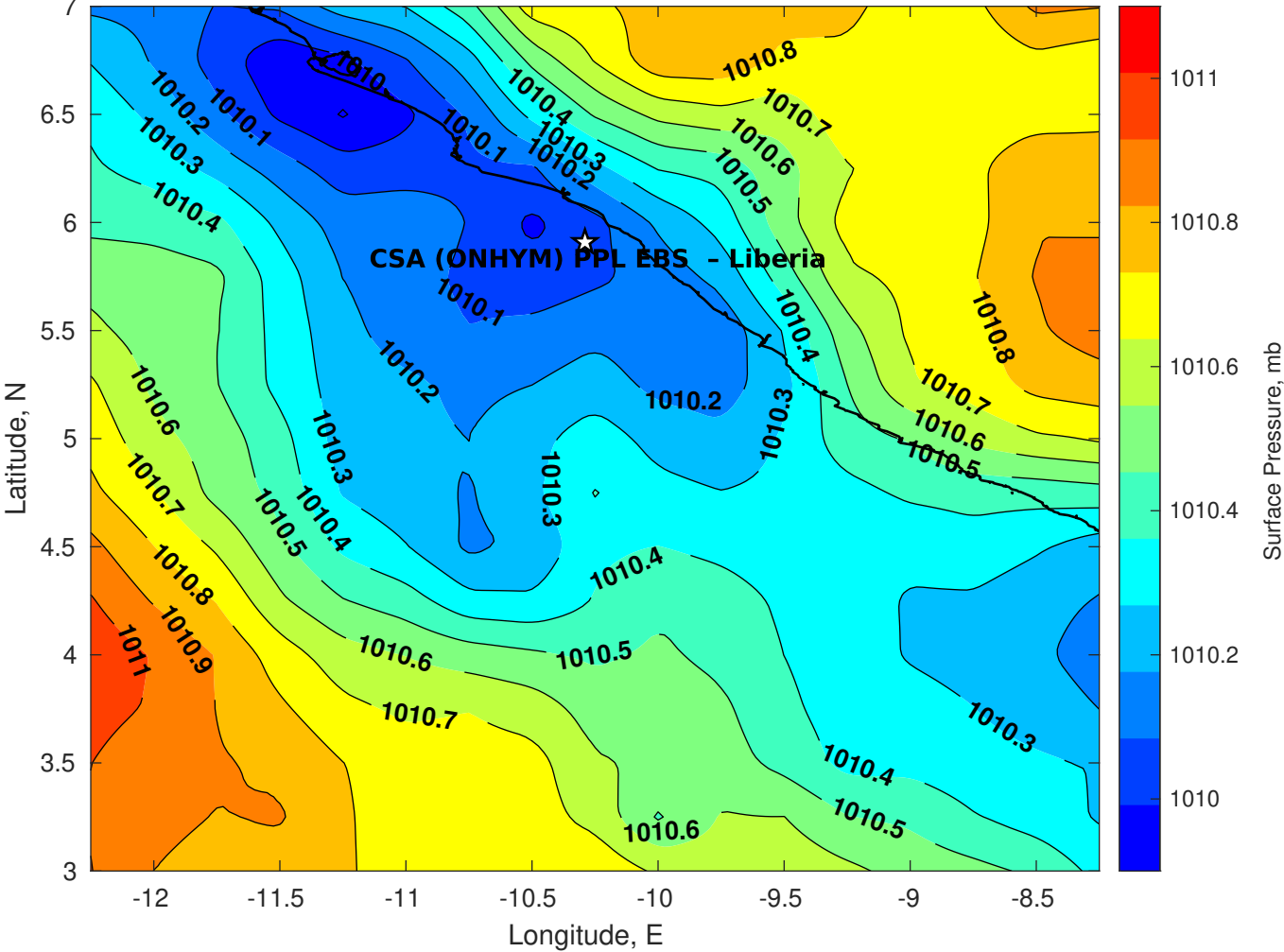
Surface Pressure (mb) for CSA (ONHYM) PPL EBS - Liberia at 19-Jan-2026 00:00:00
