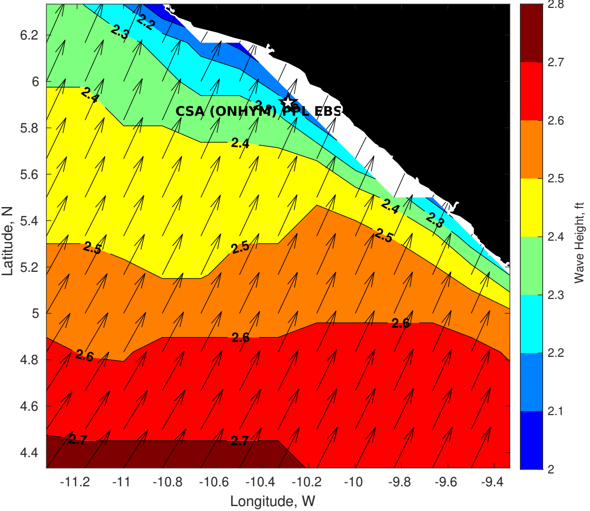
GFS Wave Height (ft) for CSA (ONHYM) PPL EBS - Liberia at 18-Jan-2026 09:00:00
