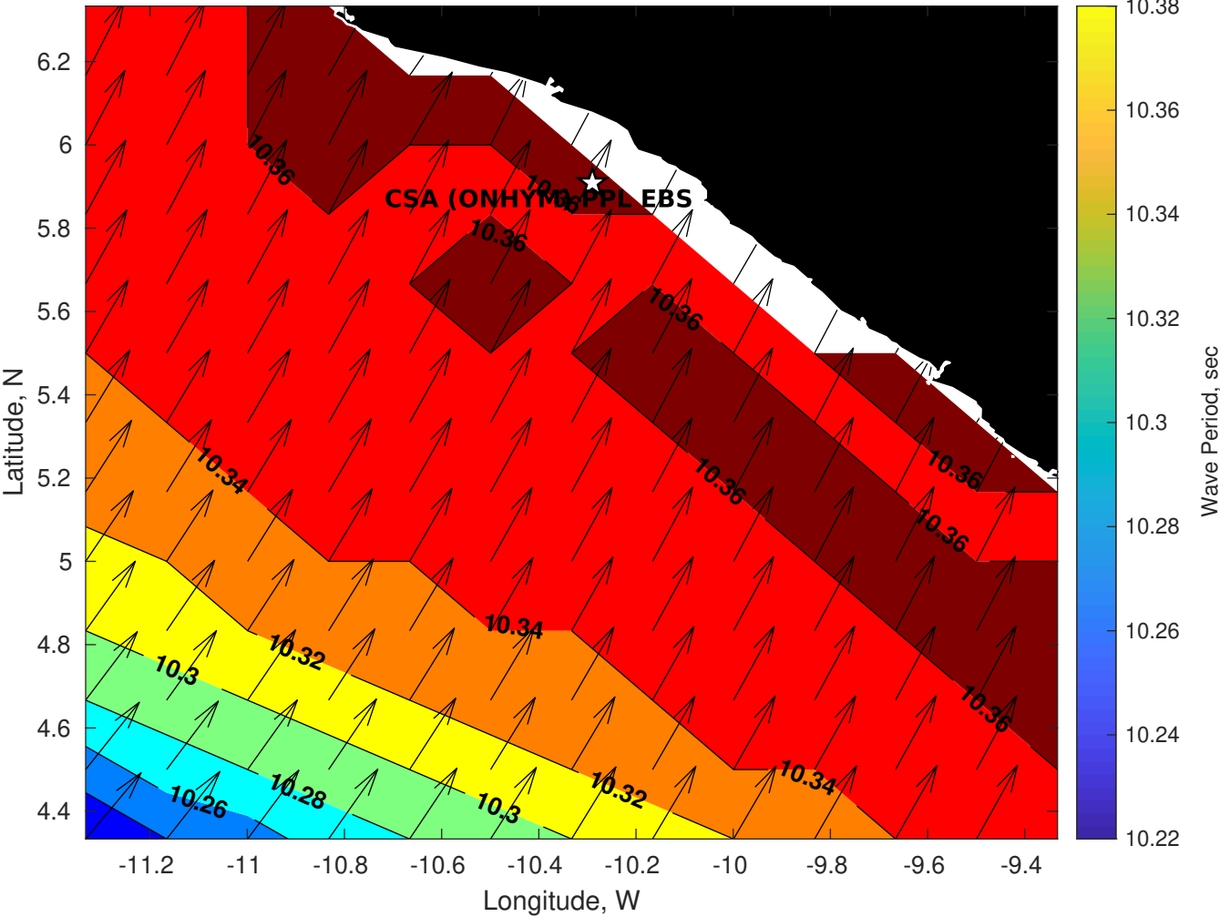
GFS Wave Period (sec) for CSA (ONHYM) PPL EBS - Liberia at 18-Jan-2026 09:00:00
