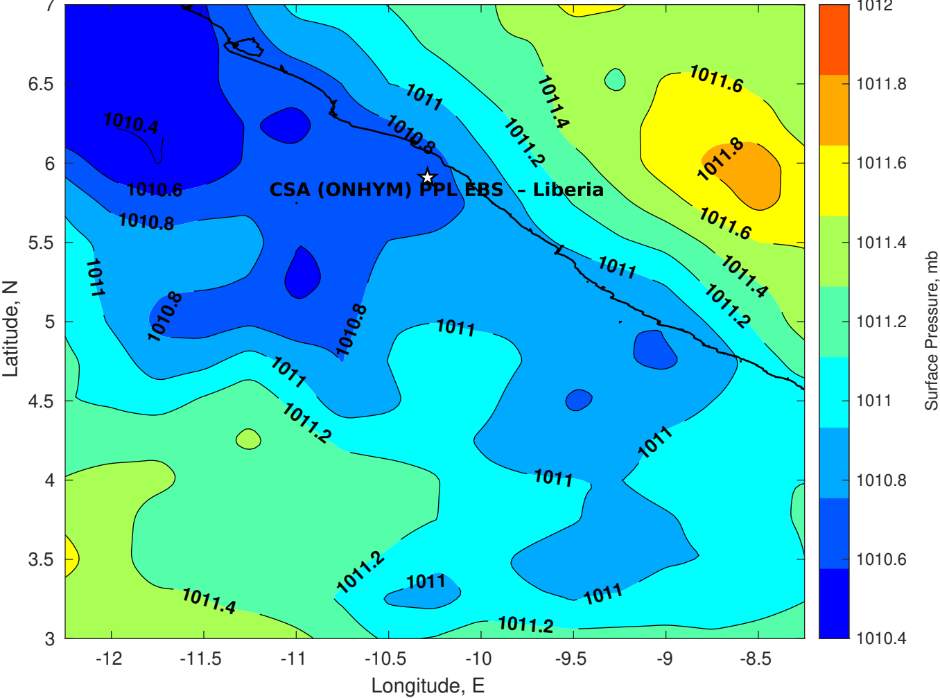
Surface Pressure (mb) for CSA (ONHYM) PPL EBS - Liberia at 18-Jan-2026 00:00:00
