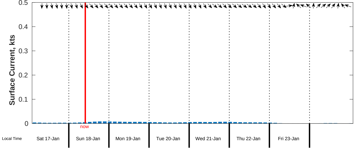
Surface Current Forecast for CSA (ONHYM) PPL EBS - Liberia from 17-Jan-2026 00:00:00 to 25-Jan-2026 00:00:00
