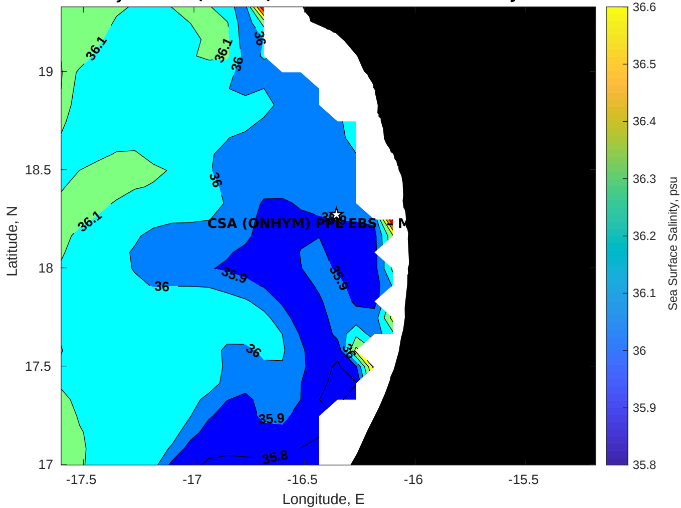
Surface Salinity for CSA (ONHYM) PPL EBS - Mauritania at 17-Jan-2026 00:00:00
