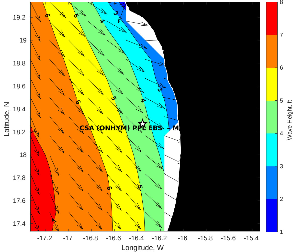
GFS Wave Height (ft) for CSA (ONHYM) PPL EBS - Mauritania at 18-Jan-2026 09:00:00
