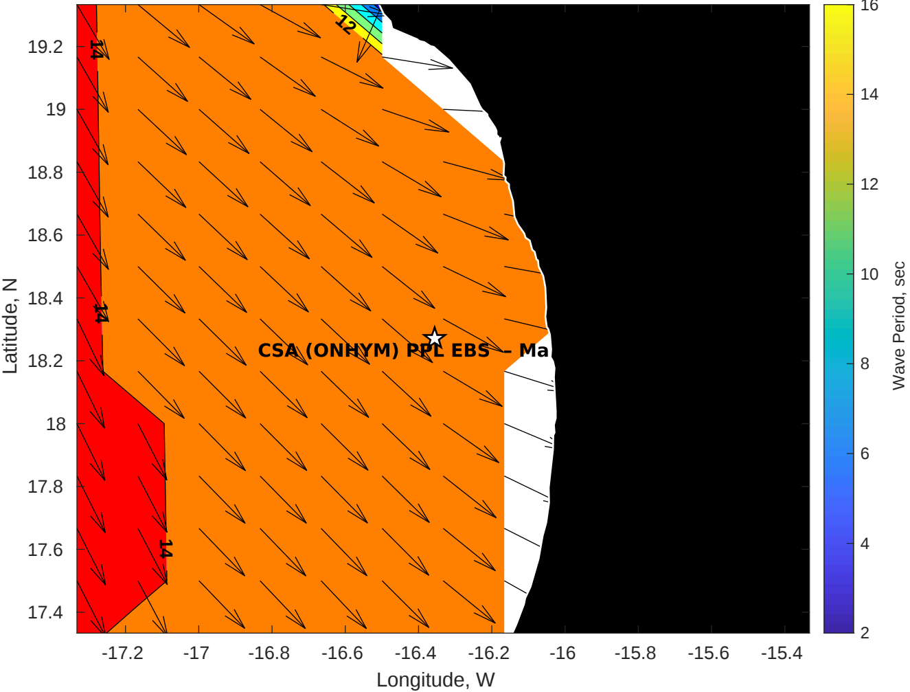
GFS Wave Period (sec) for CSA (ONHYM) PPL EBS - Mauritania at 18-Jan-2026 09:00:00
