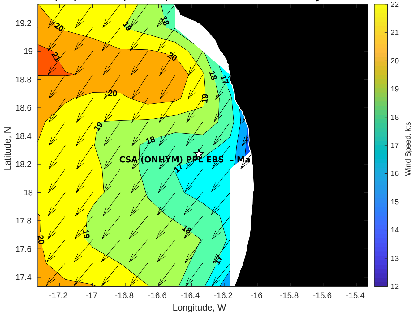
GFS Winds (kts) for CSA (ONHYM) PPL EBS - Mauritania at 18-Jan-2026 09:00:00
