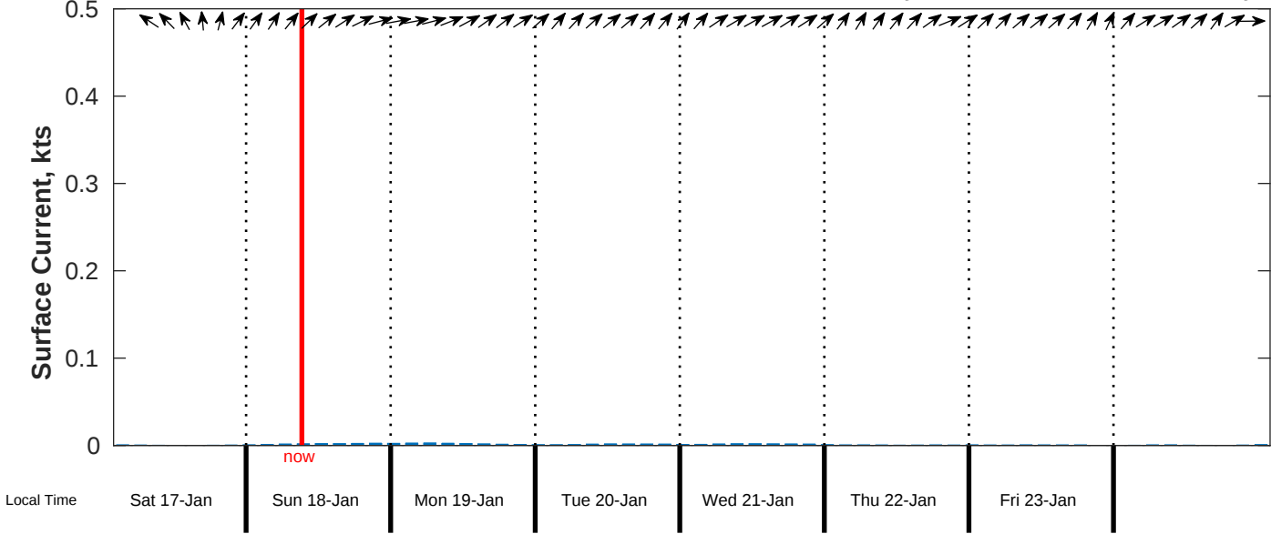
Surface Current Forecast for CSA (ONHYM) PPL EBS - Mauritania from 17-Jan-2026 00:00:00 to 25-Jan-2026 00:00:00
